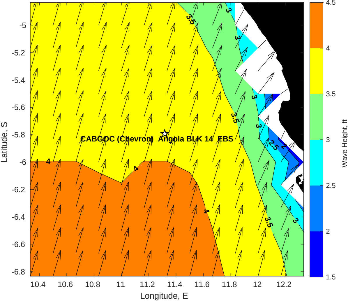
Wave Height (ft) for CABGOC (Chevron) Angola BLK 14 EBS at 06-Apr-2025 09:00:00
