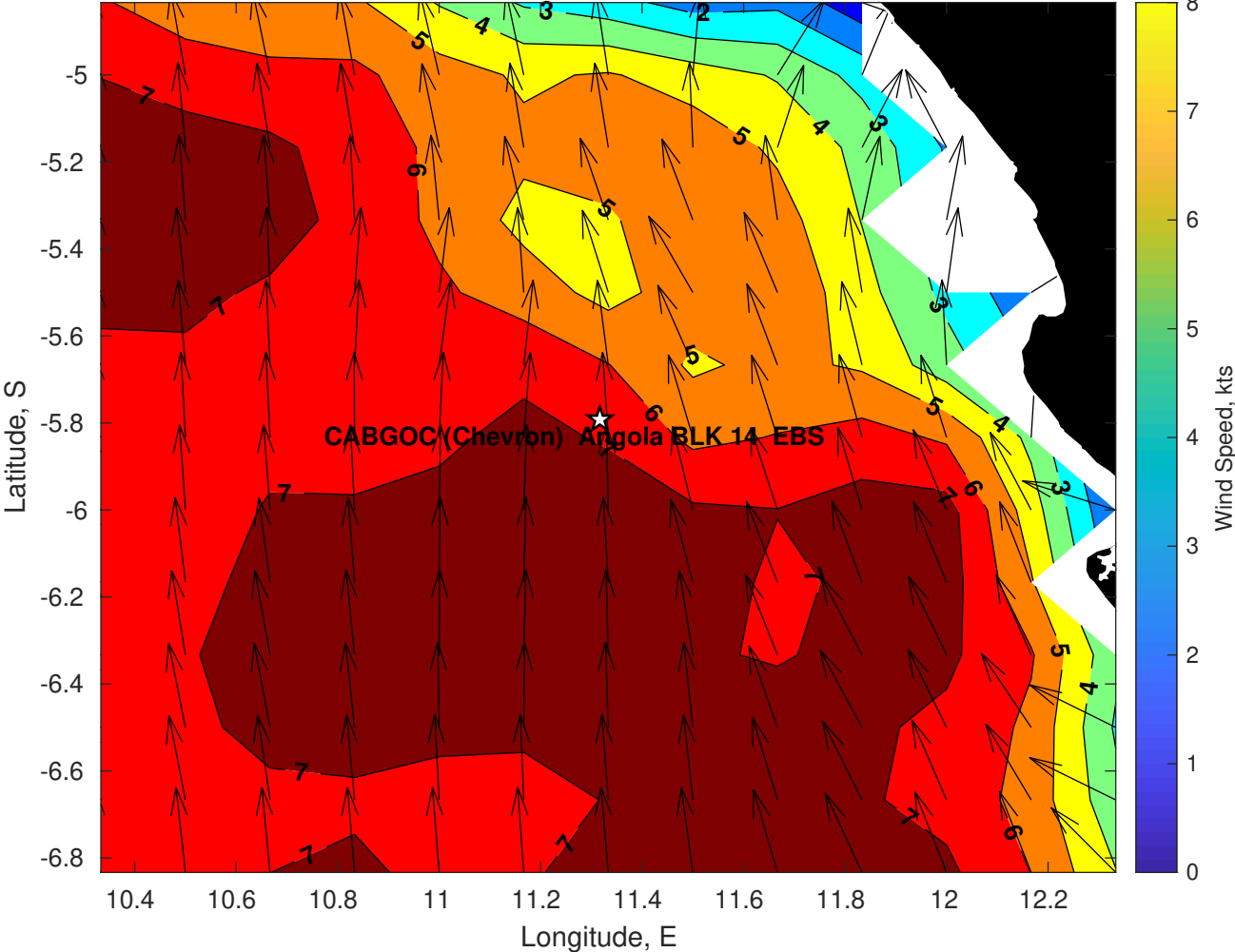
Winds (kts) for CABGOC (Chevron) Angola BLK 14 EBS at 06-Apr-2025 09:00:00
