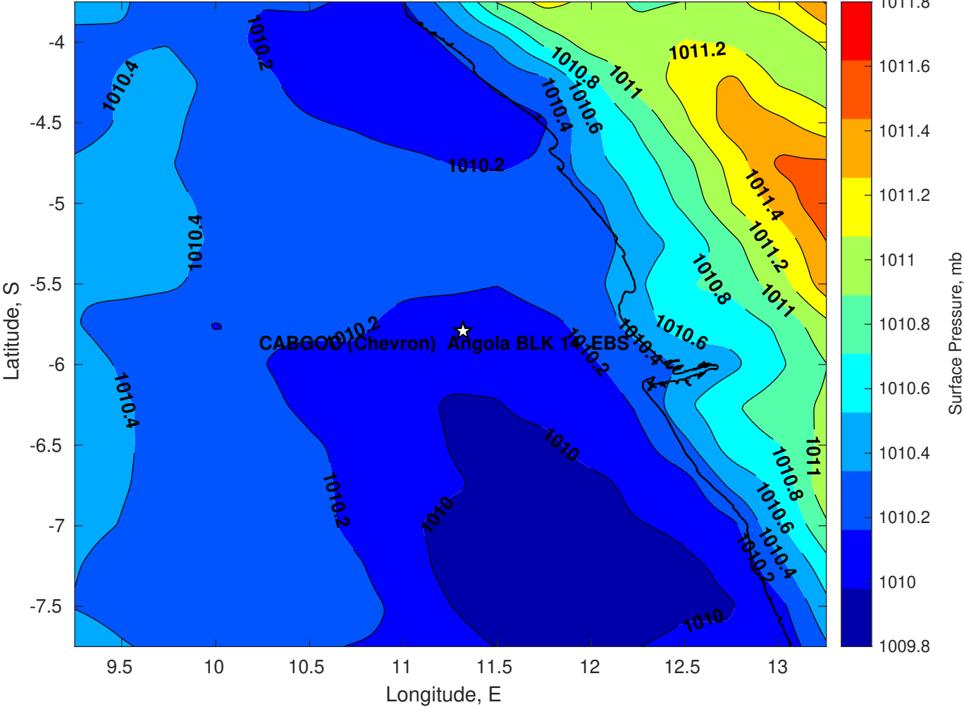
Surface Pressure (mb) for CABGOC (Chevron) Angola BLK 14 EBS at 06-Apr-2025 00:00:00
