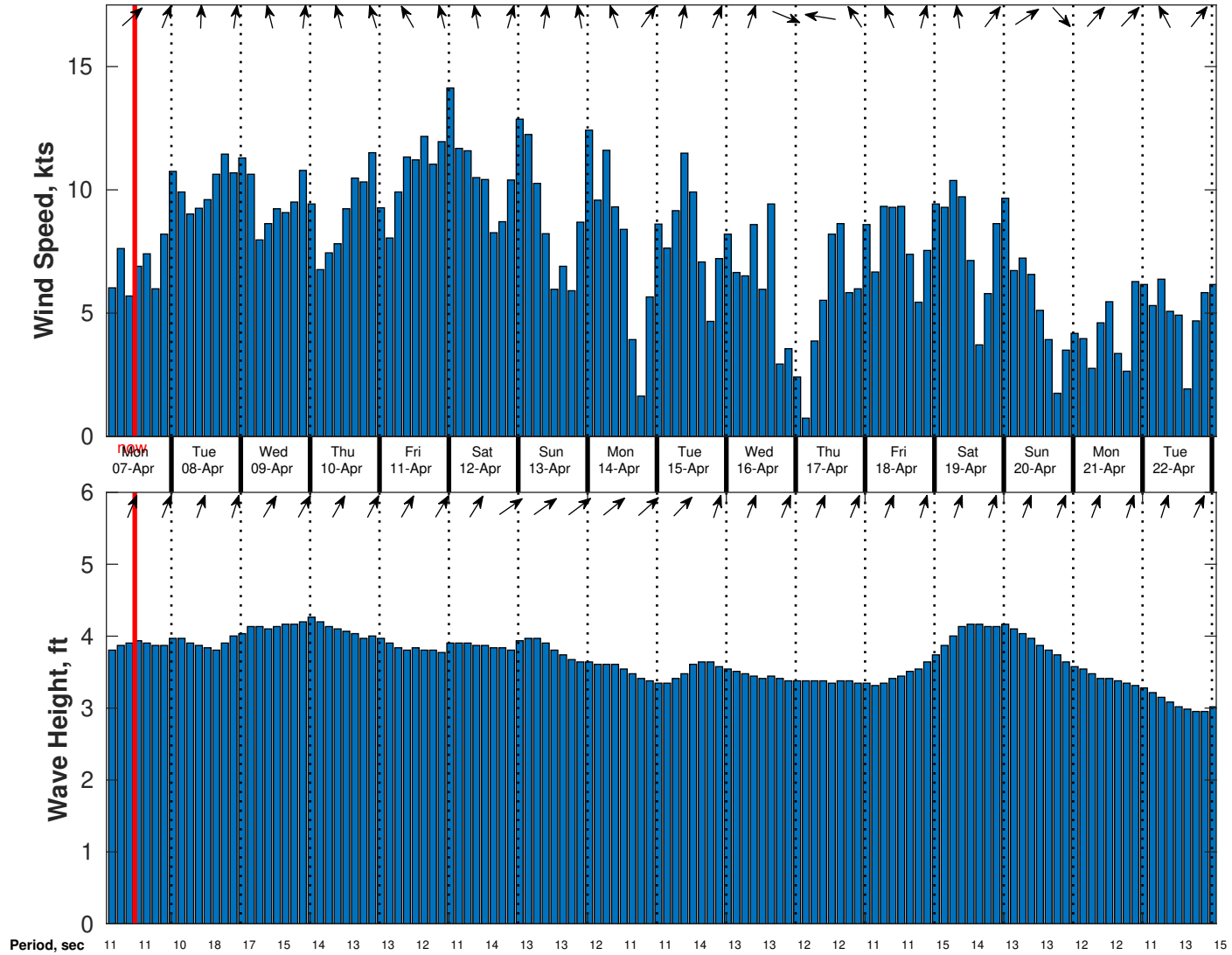
Wind & Wave Forecast for CABGOC (Chevron) Angola BLK 14 EBS from 06-Apr-2025 02:00:00 to 22-Apr-2025 02:00:00
