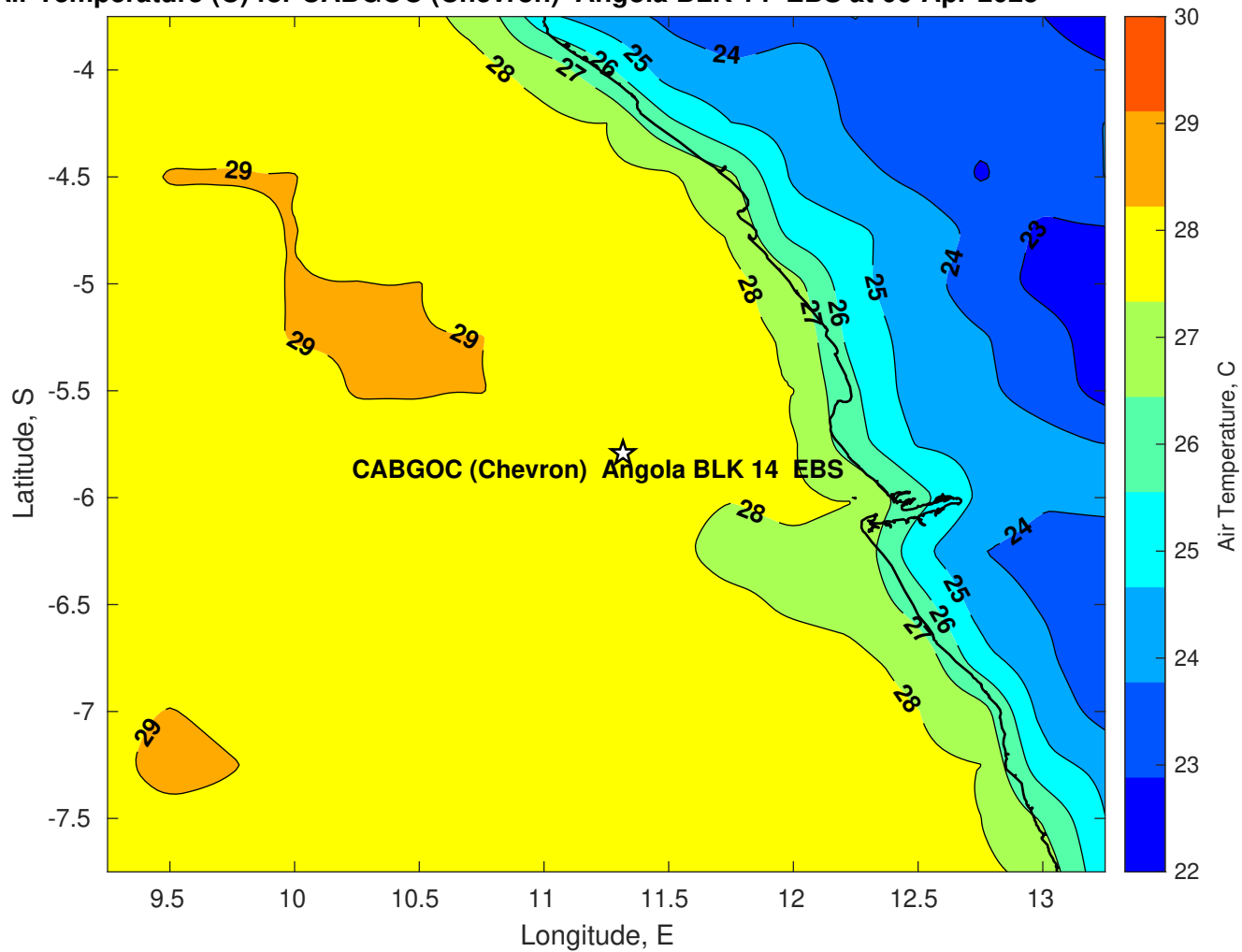
Air Temperature (C) for CABGOC (Chevron) Angola BLK 14 EBS at 06-Apr-2025
