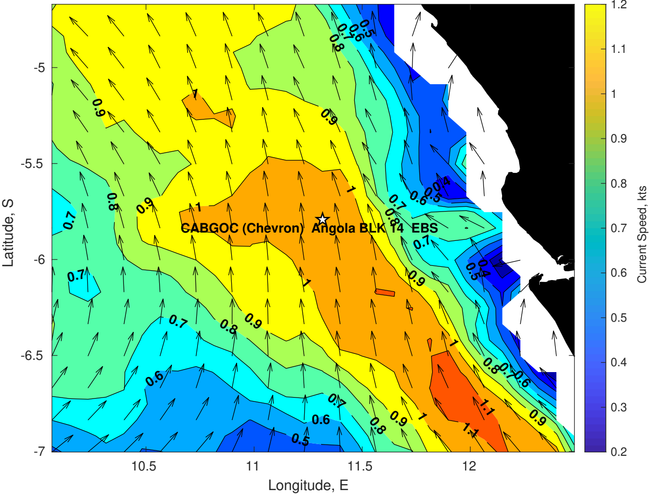
Surface Currents for CABGOC (Chevron) Angola BLK 14 EBS at 05-Apr-2025 00:00:00
