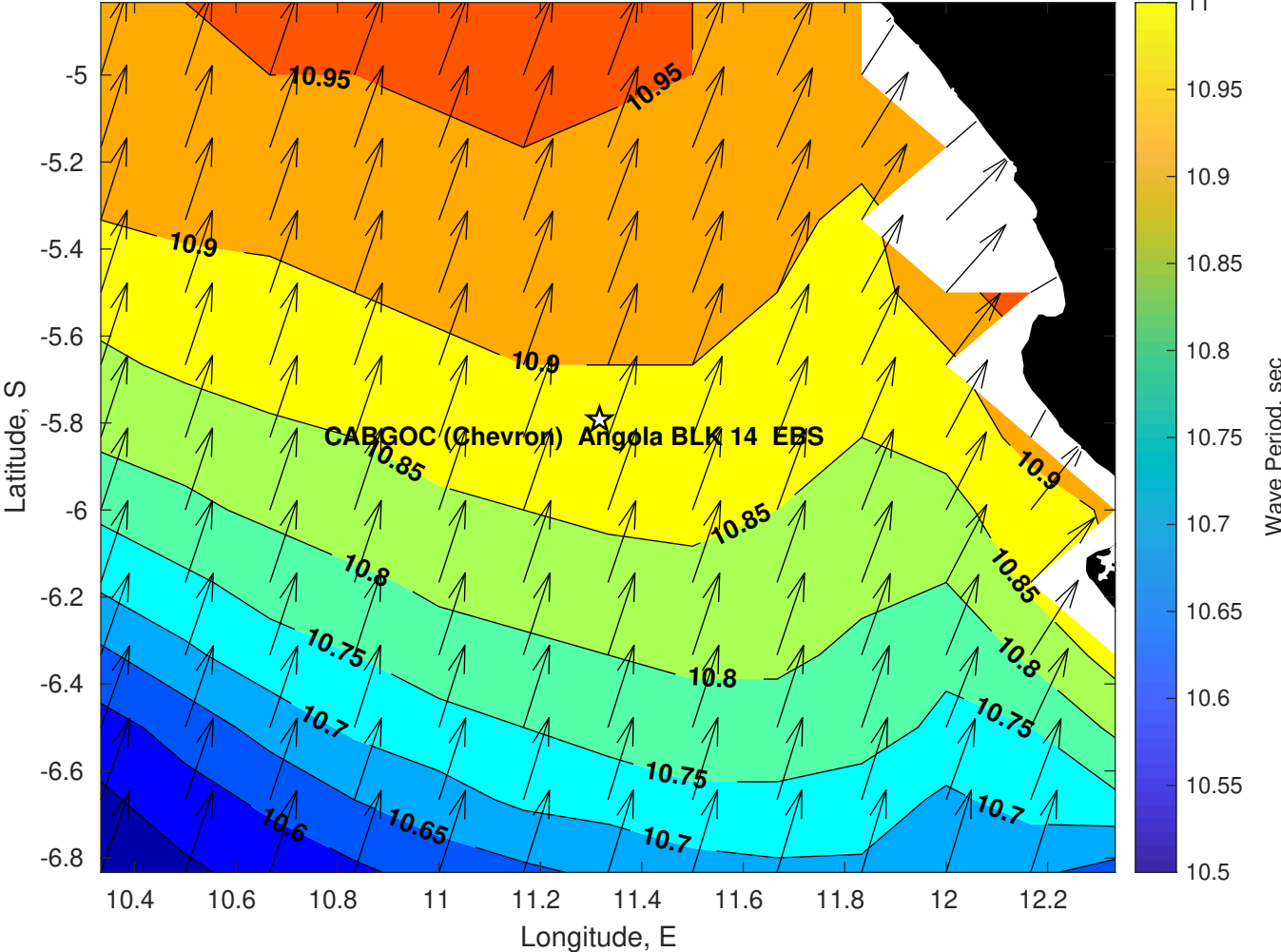
Wave Period (sec) for CABGOC (Chevron) Angola BLK 14 EBS at 06-Apr-2025 09:00:00
