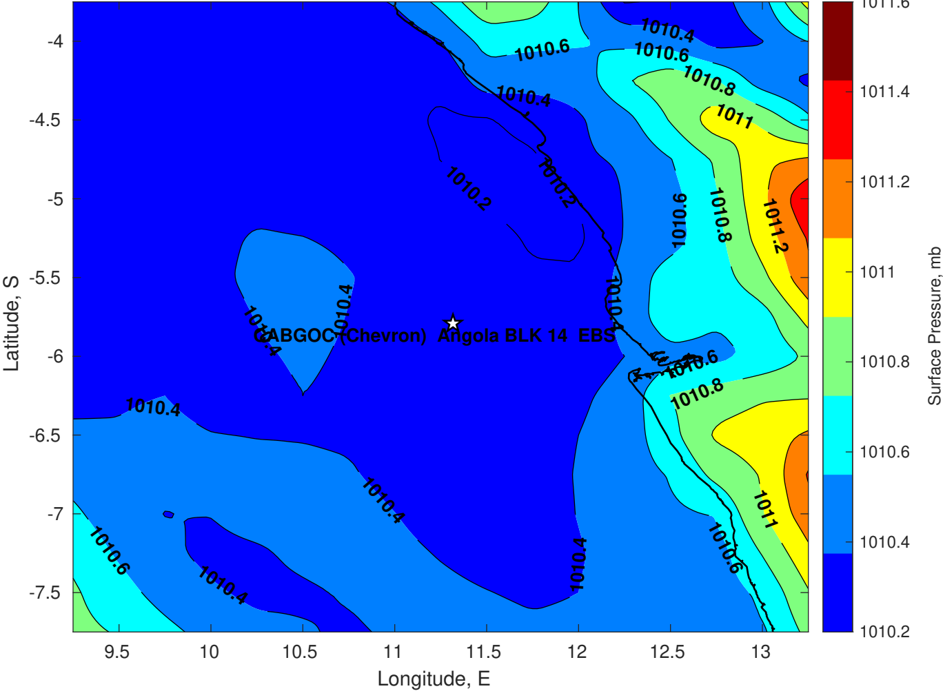
Surface Pressure (mb) for CABGOC (Chevron) Angola BLK 14 EBS at 07-Apr-2025 00:00:00
