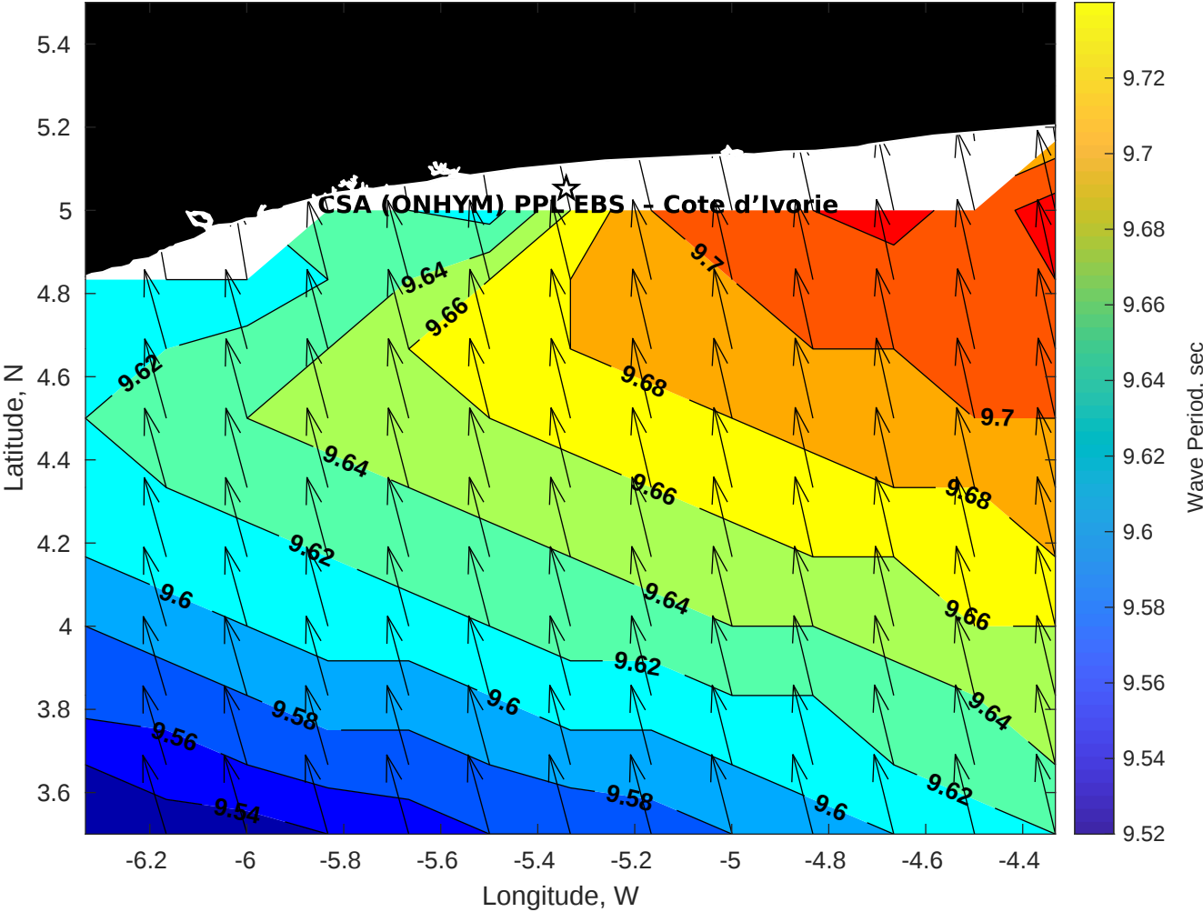
Wave Period (sec) for CSA (ONHYM) PPL EBS - Cote d'Ivoire at 06-Apr-2025 09:00:00
