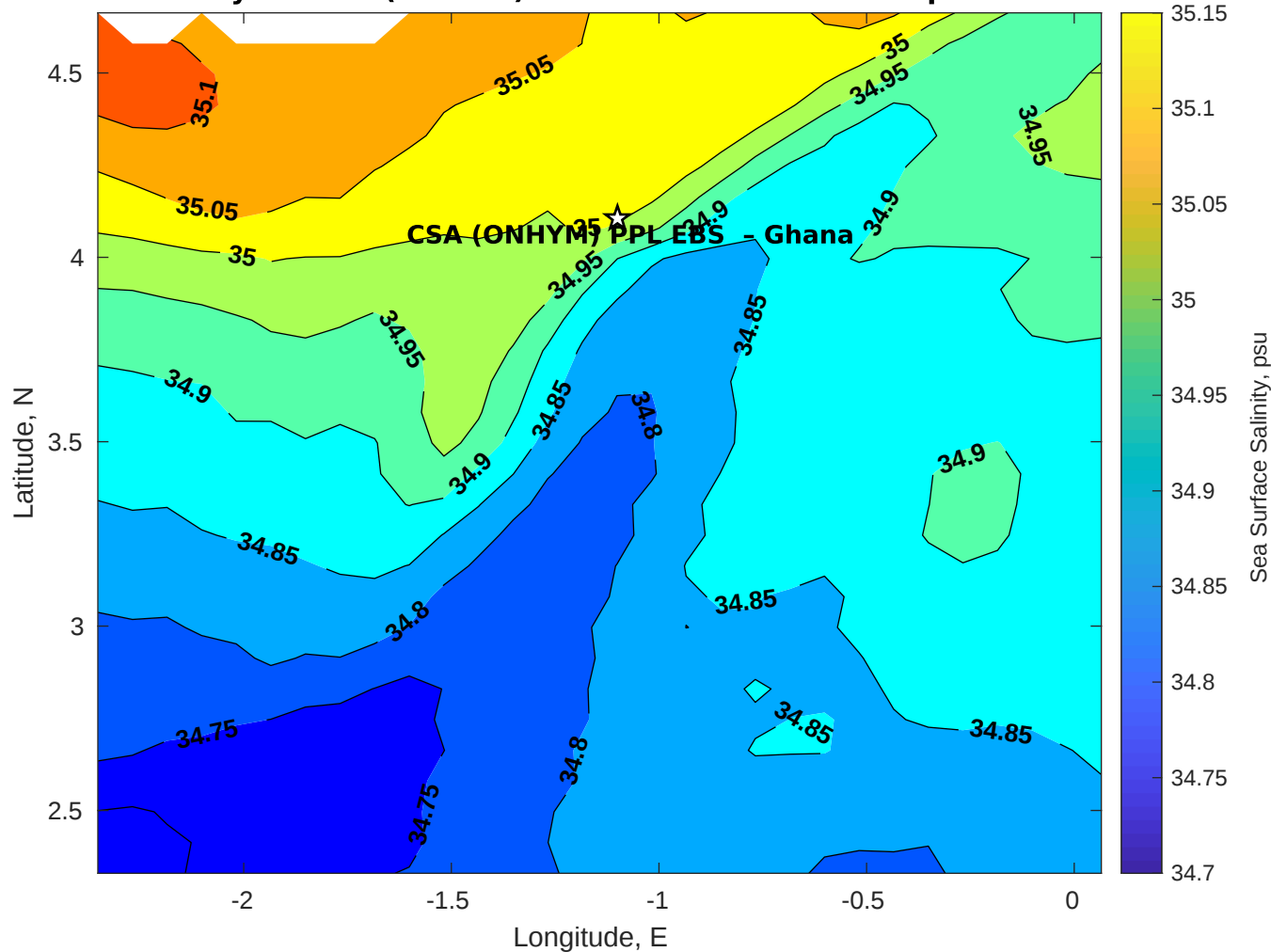
Surface Salinity for CSA (ONHYM) PPL EBS - Ghana at 05-Apr-2025 00:00:00
