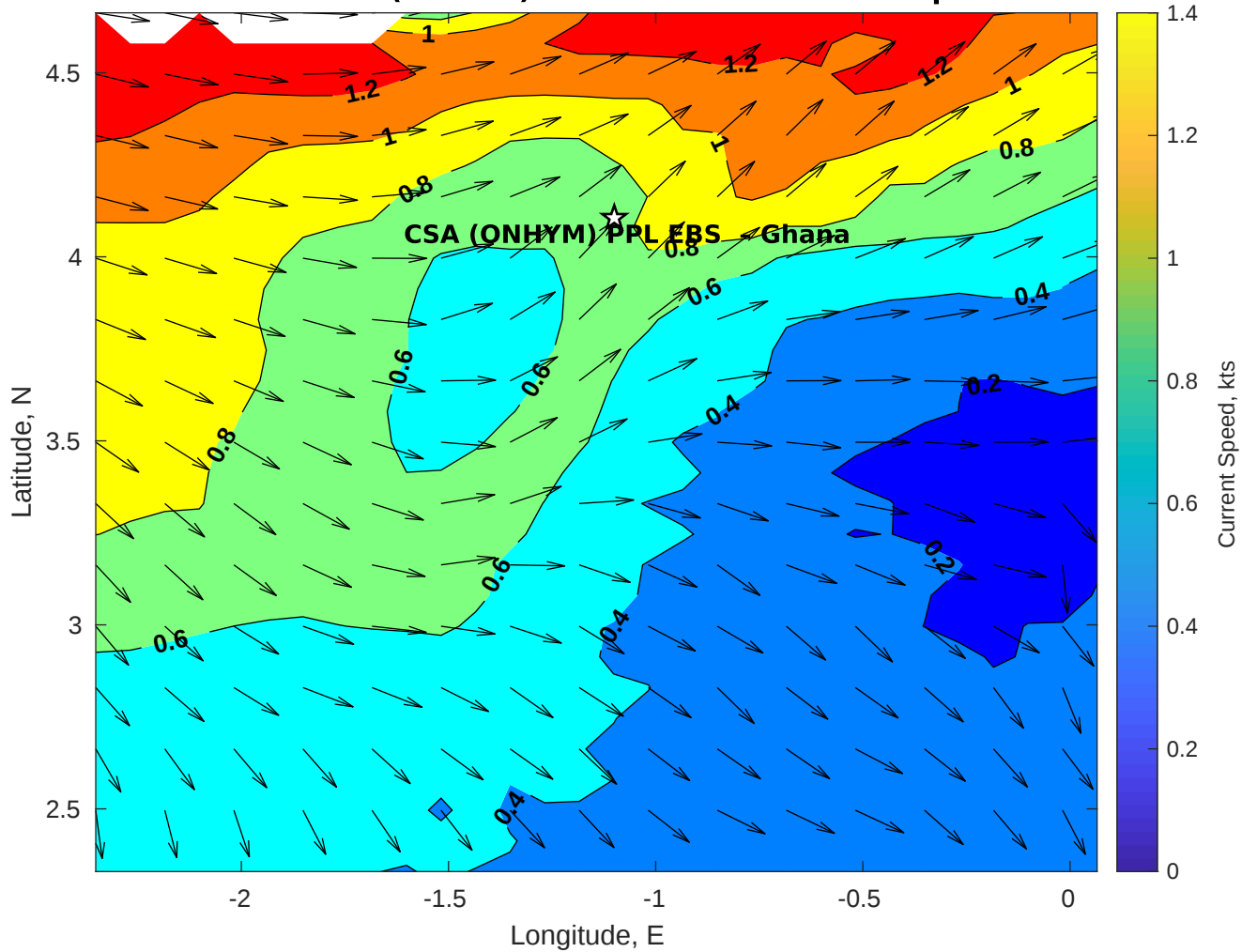
Surface Currents for CSA (ONHYM) PPL EBS - Ghana at 05-Apr-2025 00:00:00
