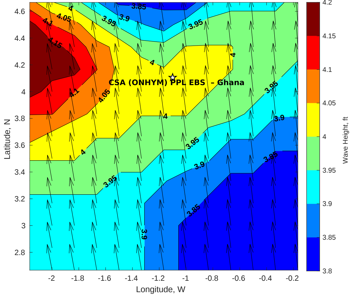
Wave Height (ft) for CSA (ONHYM) PPL EBS - Ghana at 06-Apr-2025 09:00:00
