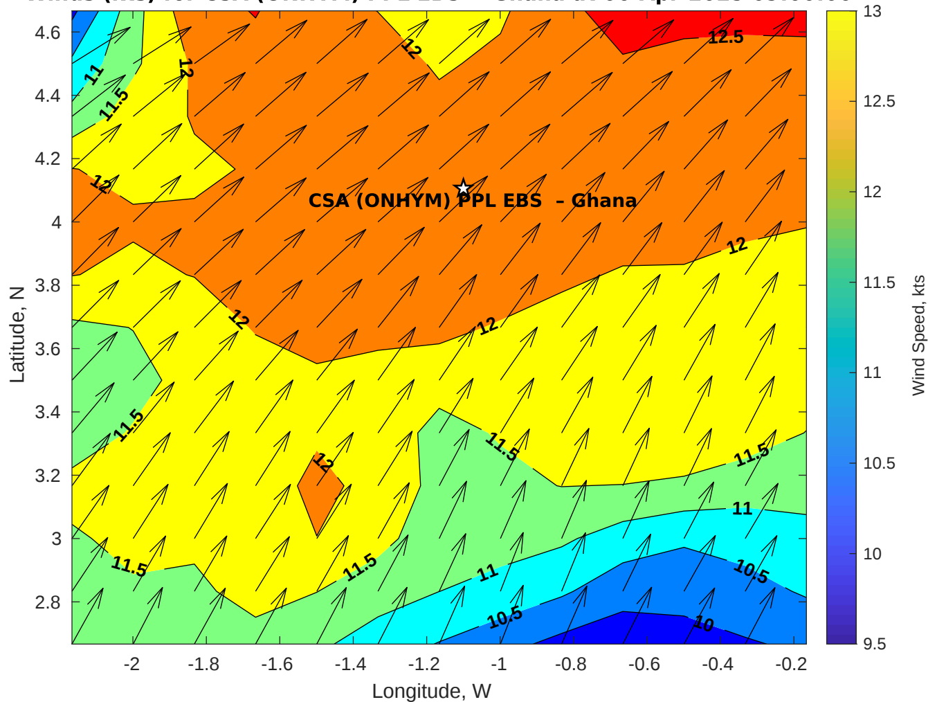
Winds (kts) for CSA (ONHYM) PPL EBS - Ghana at 06-Apr-2025 09:00:00
