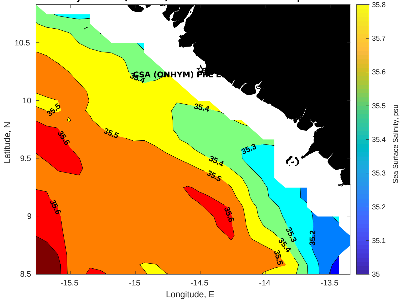
Surface Salinity for CSA (ONHYM) PPL EBS - Guinea at 05-Apr-2025 00:00:00
