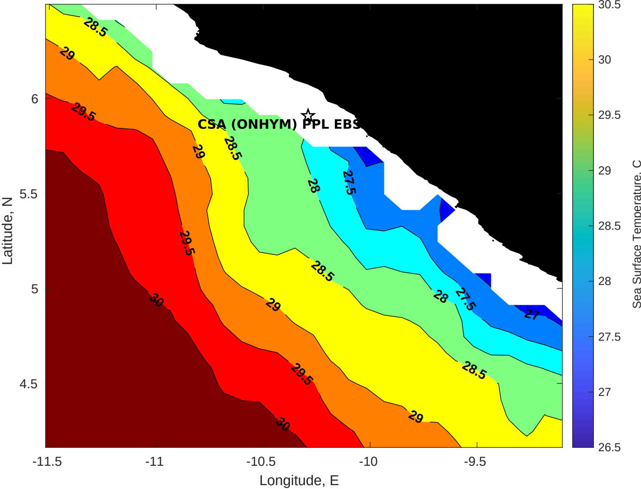
SST for CSA (ONHYM) PPL EBS - Liberia at 05-Apr-2025 00:00:00
