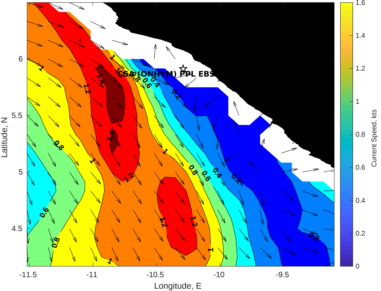
Surface Currents for CSA (ONHYM) PPL EBS - Liberia at 05-Apr-2025 00:00:00
