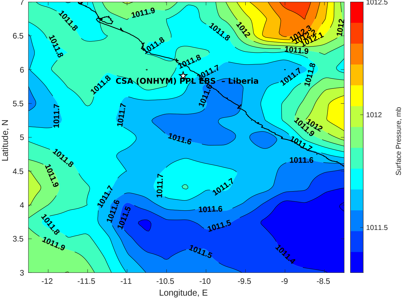
Surface Pressure (mb) for CSA (ONHYM) PPL EBS - Liberia at 08-Apr-2025 00:00:00
