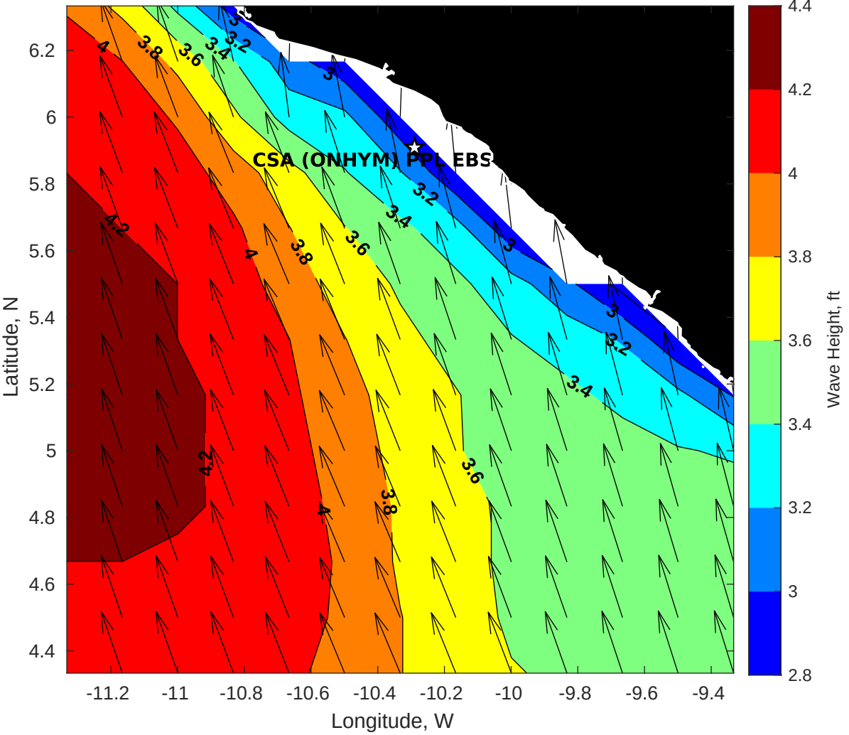
Wave Height (ft) for CSA (ONHYM) PPL EBS - Liberia at 06-Apr-2025 09:00:00
