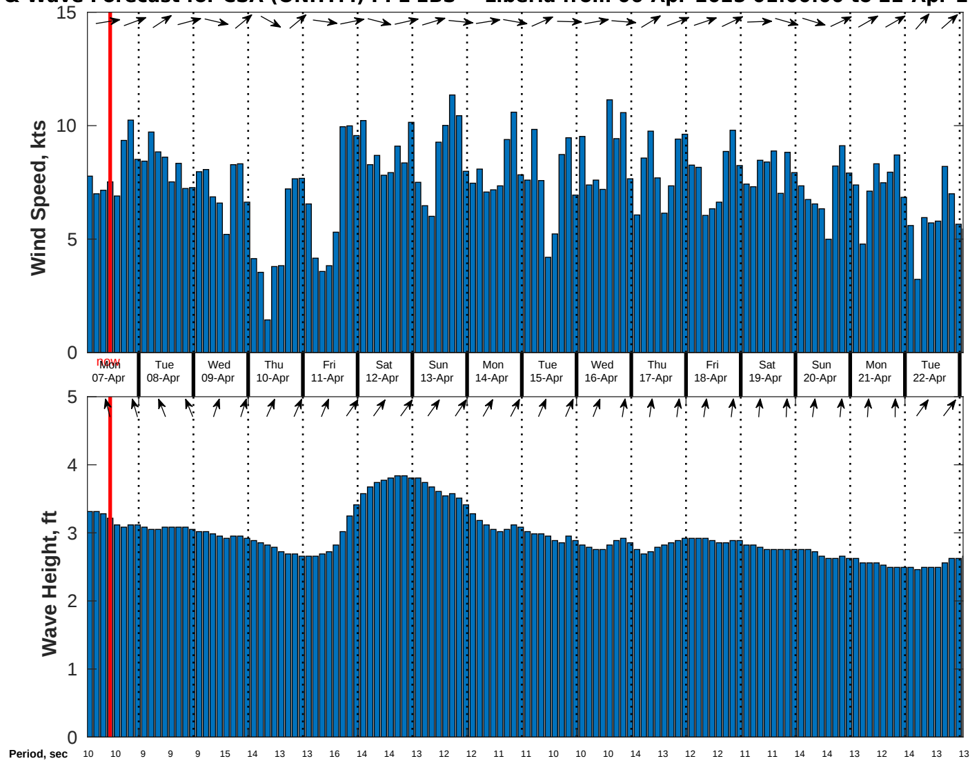
Wind & Wave Forecast for CSA (ONHYM) PPL EBS - Liberia from 06-Apr-2025 01:00:00 to 22-Apr-2025 01:00:00
