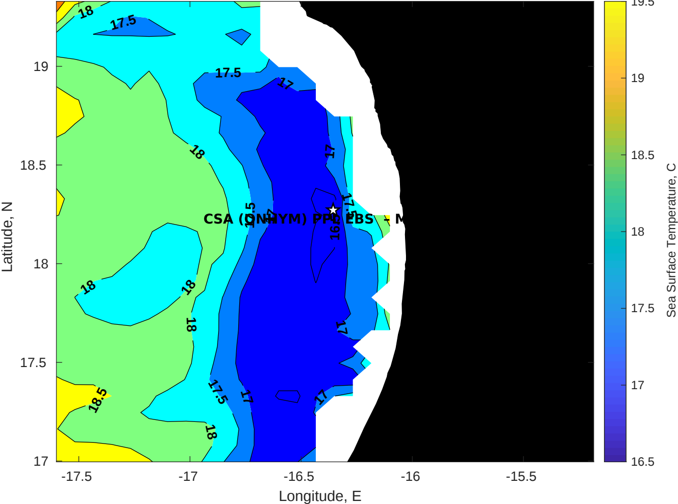
SST for CSA (ONHYM) PPL EBS - Mauritania at 05-Apr-2025 00:00:00
