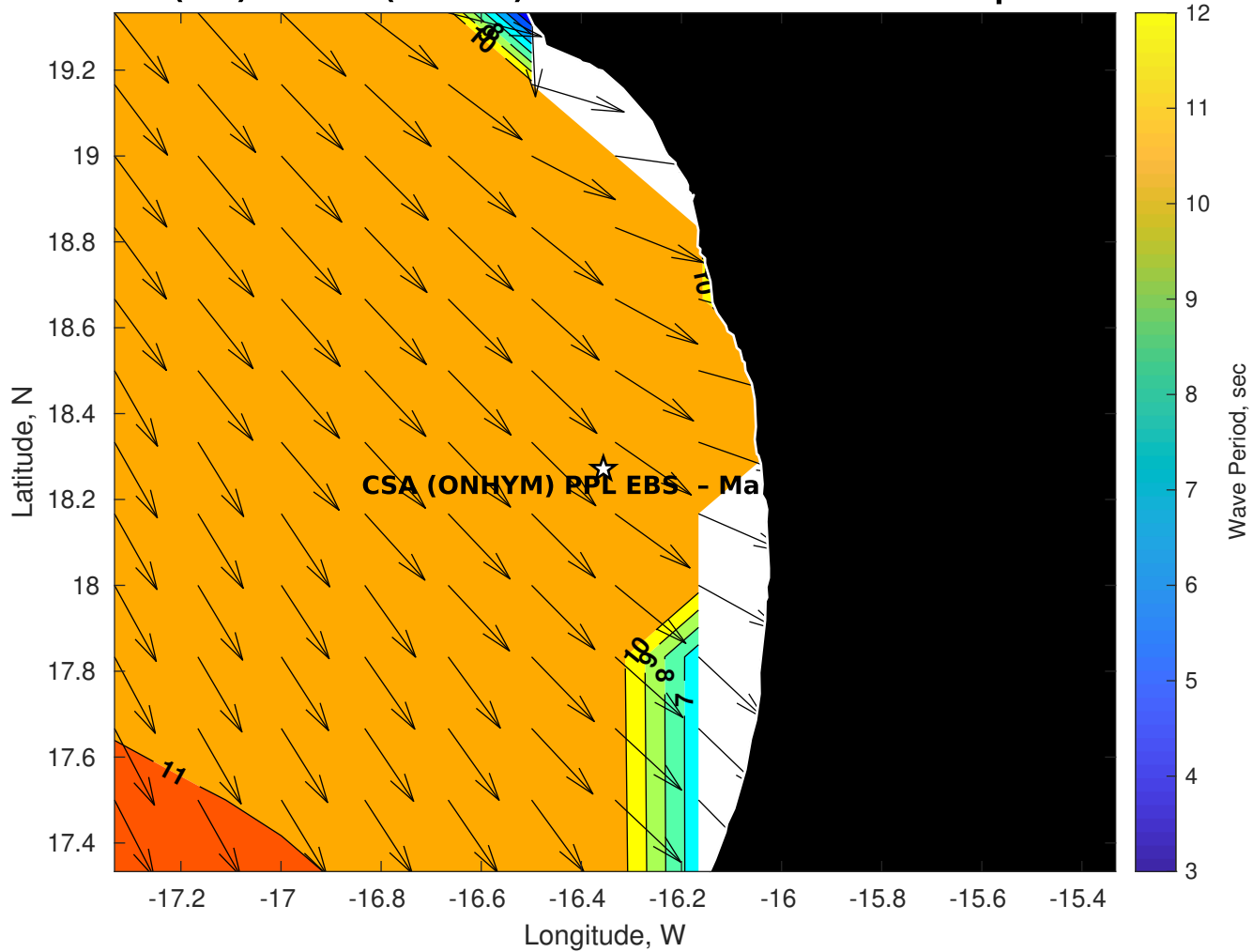
Wave Period (sec) for CSA (ONHYM) PPL EBS - Mauritania at 06-Apr-2025 09:00:00
