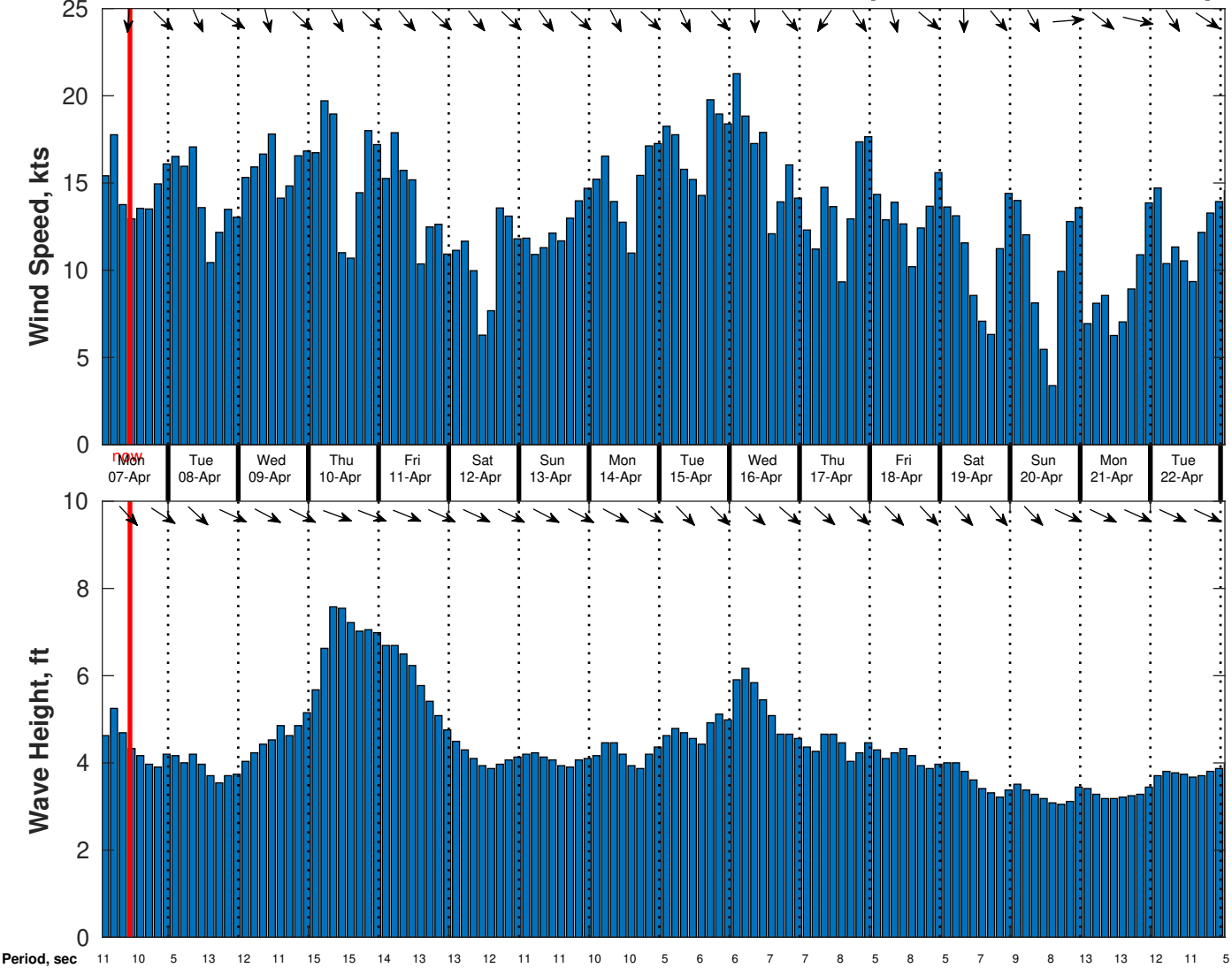
Wind & Wave Forecast for CSA (ONHYM) PPL EBS - Mauritania from 06-Apr-2025 01:00:00 to 22-Apr-2025 01:00:00
