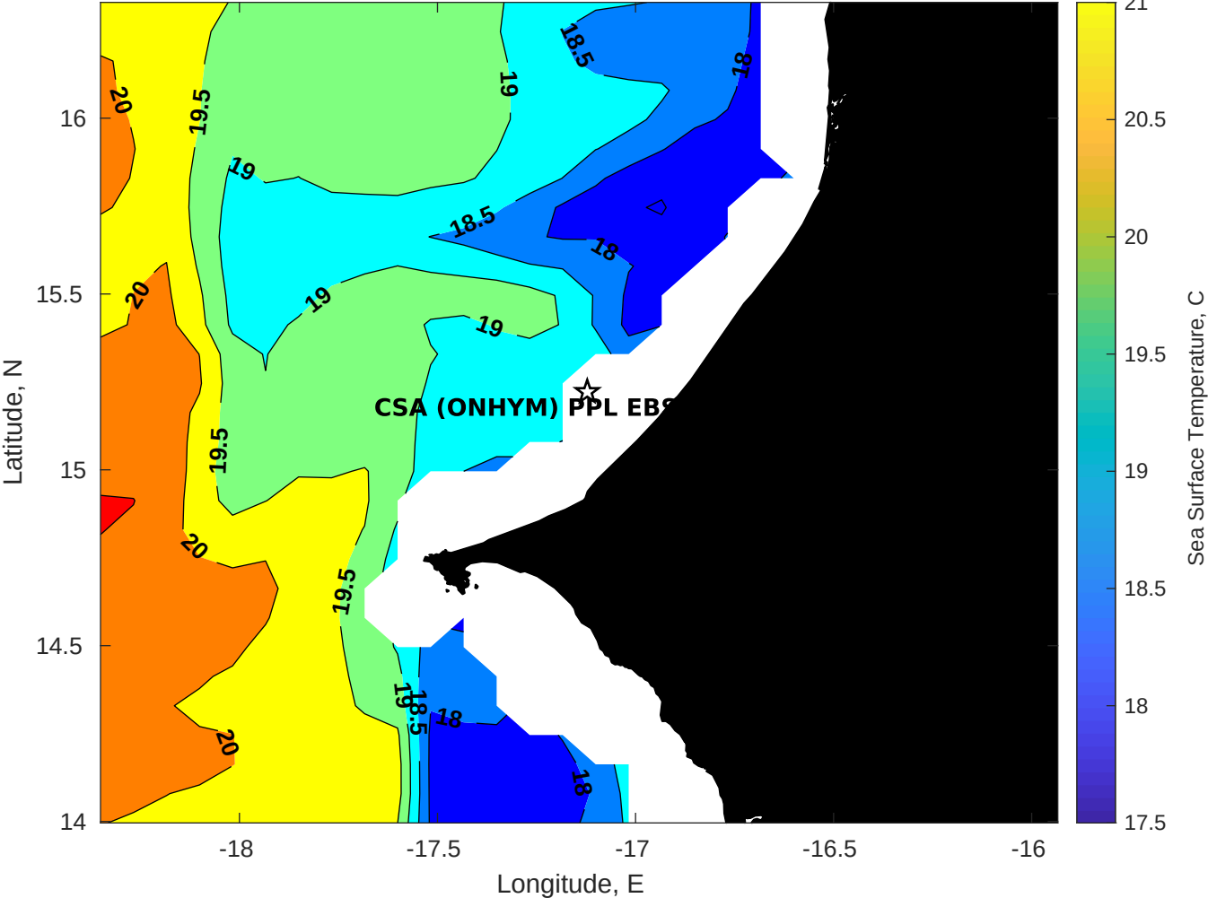
SST for CSA (ONHYM) PPL EBS - Senegal at 05-Apr-2025 00:00:00
