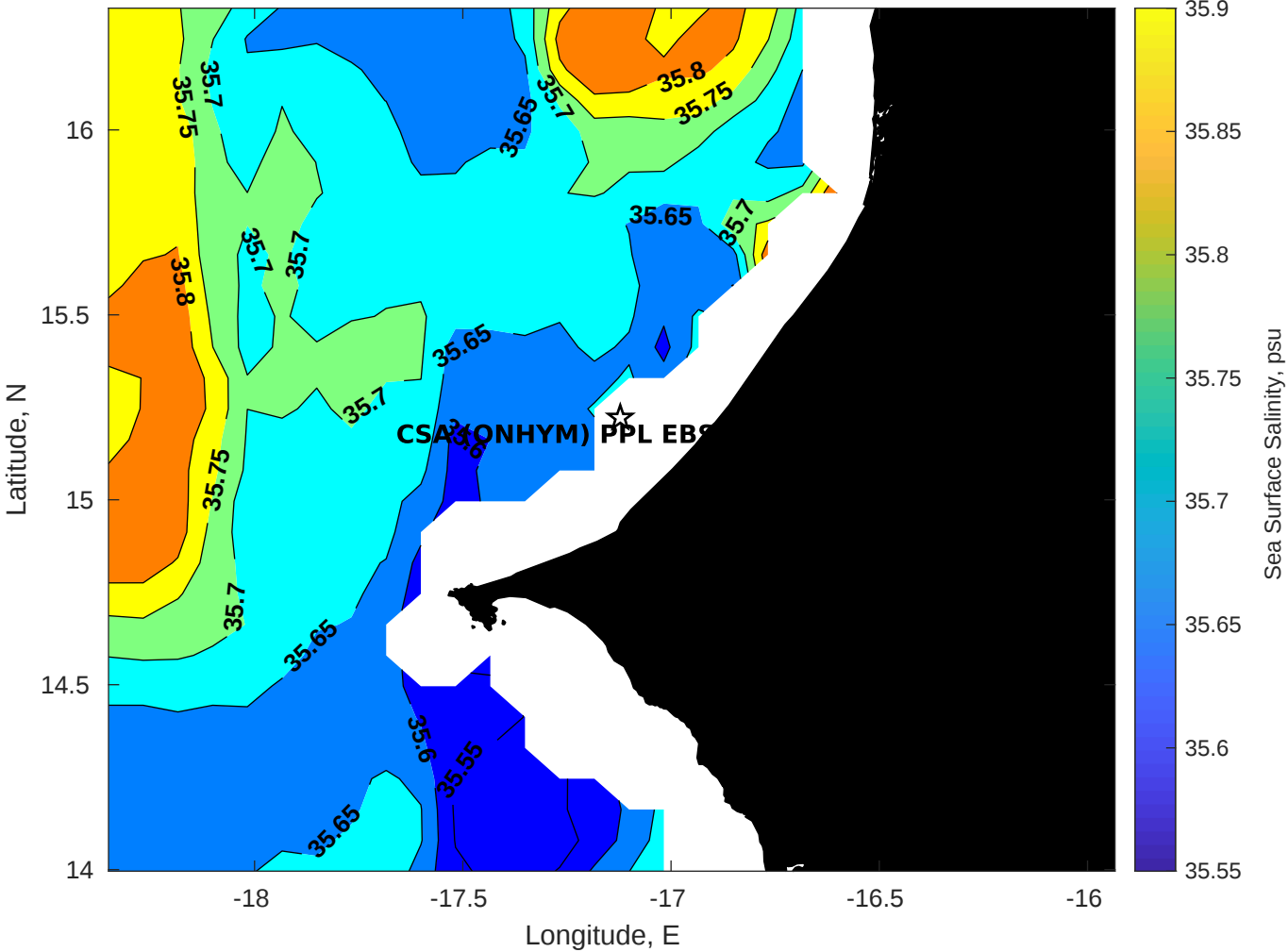
Surface Salinity for CSA (ONHYM) PPL EBS - Senegal at 05-Apr-2025 00:00:00
