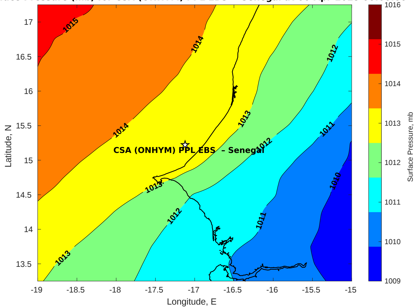
Surface Pressure (mb) for CSA (ONHYM) PPL EBS - Senegal at 06-Apr-2025 00:00:00
