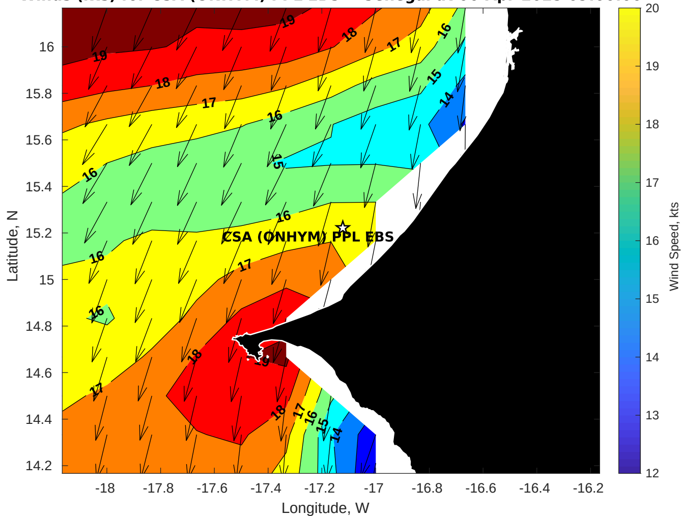
Winds (kts) for CSA (ONHYM) PPL EBS - Senegal at 06-Apr-2025 09:00:00
