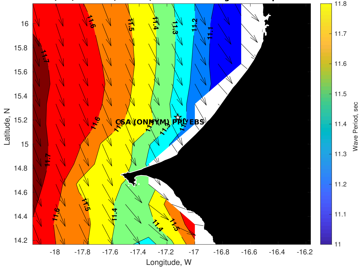
Wave Period (sec) for CSA (ONHYM) PPL EBS - Senegal at 06-Apr-2025 09:00:00
