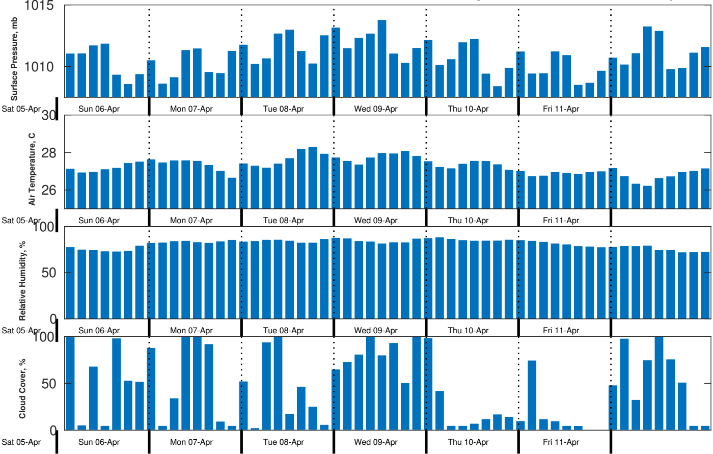
Met Forecast for CSA (ONHYM) PPL EBS - Sierra Leone from 06-Apr-2025 00:00:00 to 13-Apr-2025 00:00:00
