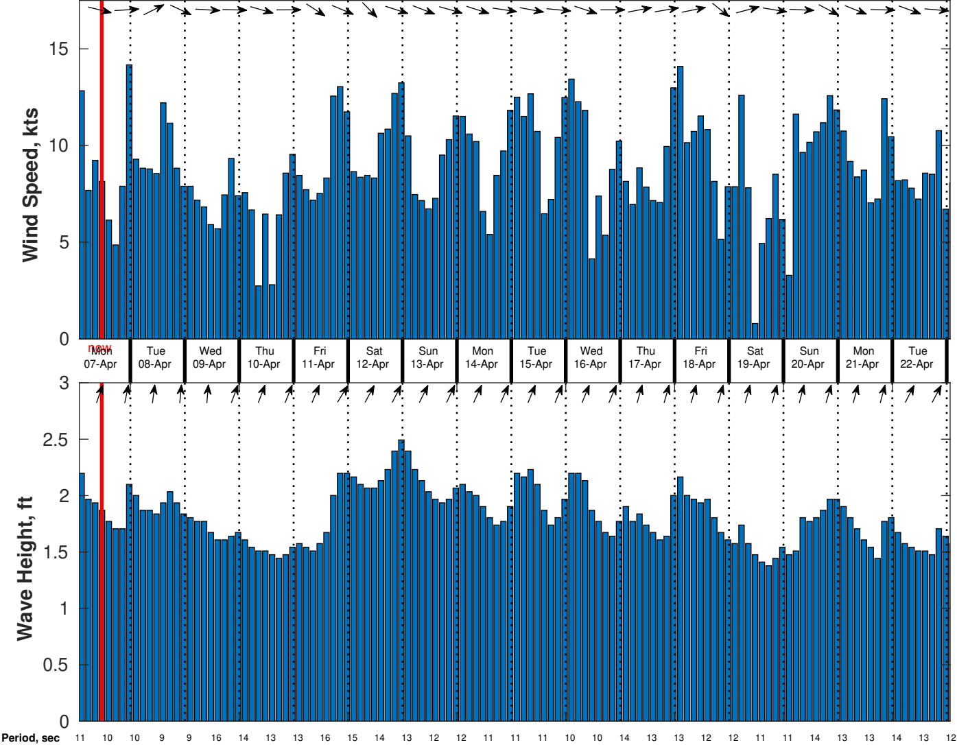
Wind & Wave Forecast for CSA (ONHYM) PPL EBS - Sierra Leone from 06-Apr-2025 01:00:00 to 22-Apr-2025 01:00:00
