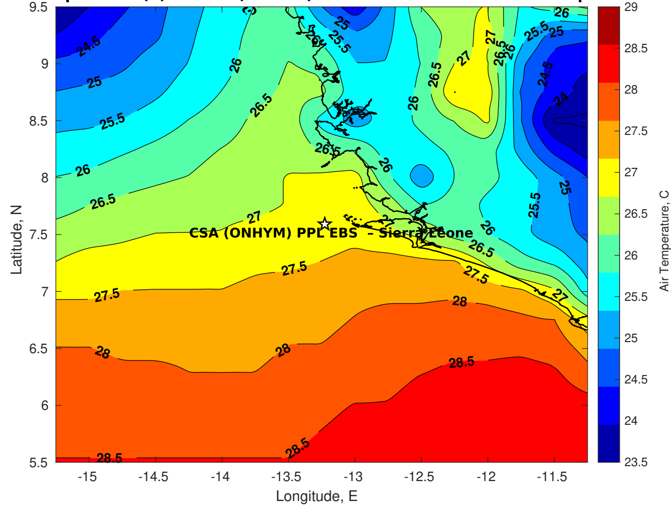
Air Temperature (C) for CSA (ONHYM) PPL EBS - Sierra Leone at 06-Apr-2025
