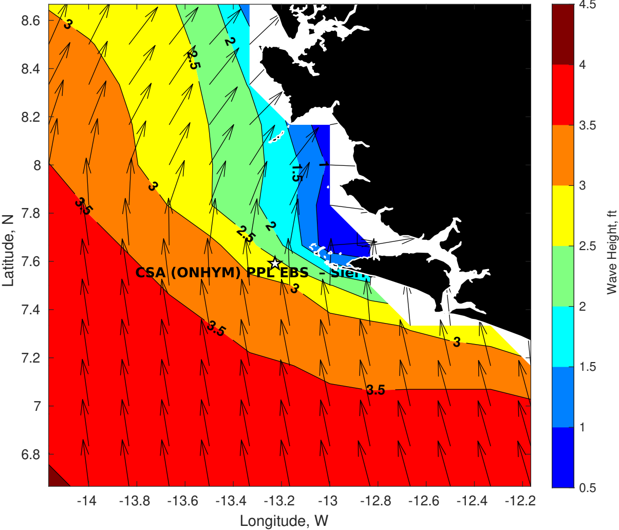
Wave Height (ft) for CSA (ONHYM) PPL EBS - Sierra Leone at 06-Apr-2025 09:00:00
