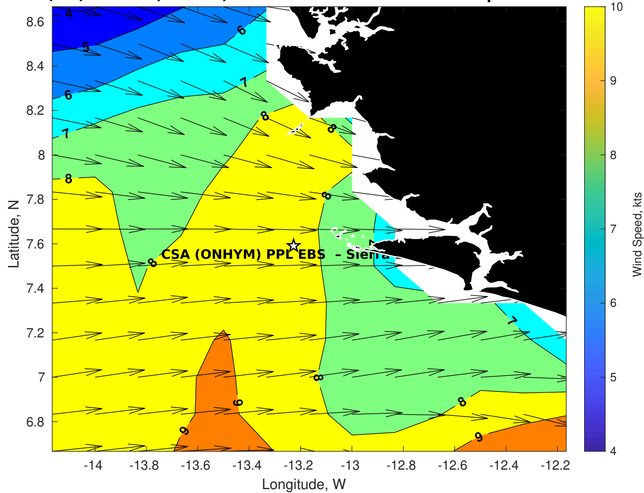
Winds (kts) for CSA (ONHYM) PPL EBS - Sierra Leone at 06-Apr-2025 09:00:00
