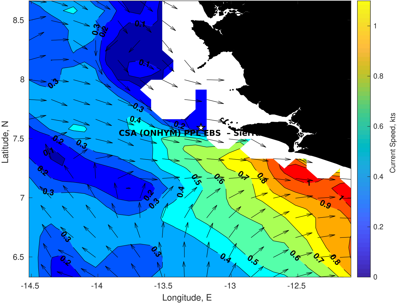
Surface Currents for CSA (ONHYM) PPL EBS - Sierra Leone at 05-Apr-2025 00:00:00
