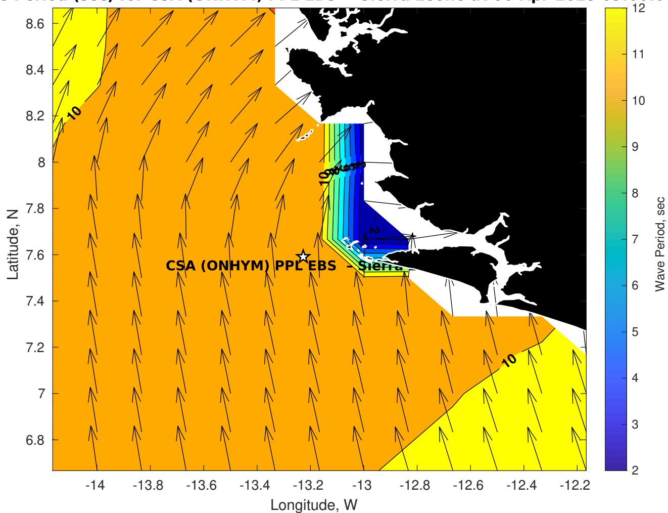
Wave Period (sec) for CSA (ONHYM) PPL EBS - Sierra Leone at 06-Apr-2025 09:00:00
