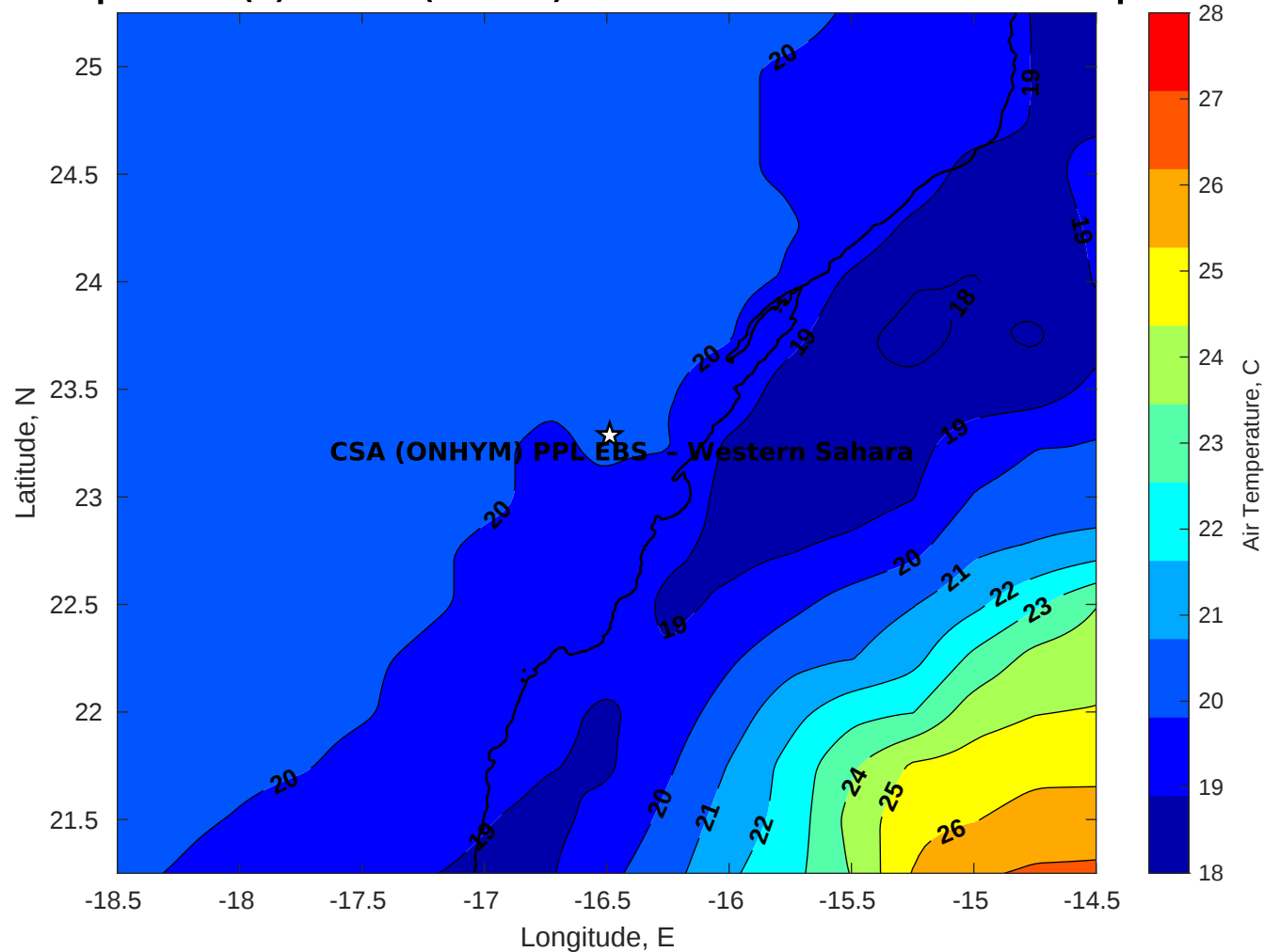
Air Temperature (C) for CSA (ONHYM) PPL EBS - Western Sahara at 06-Apr-2025
