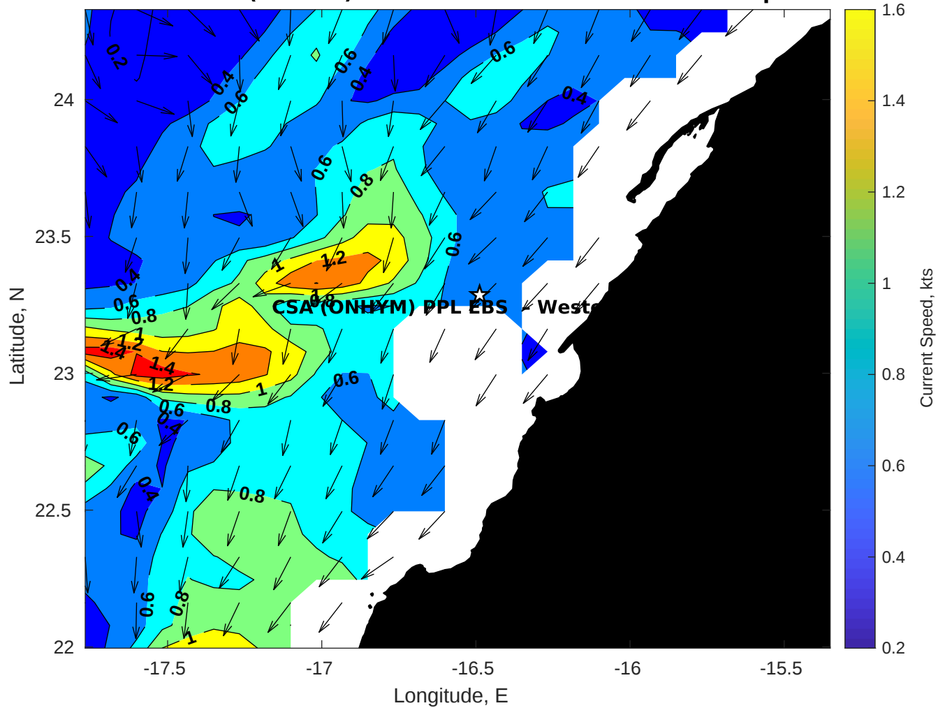
Surface Currents for CSA (ONHYM) PPL EBS - Western Sahara at 05-Apr-2025 00:00:00
