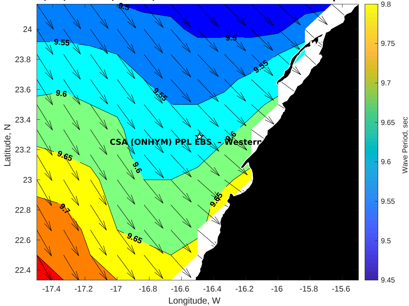
Wave Period (sec) for CSA (ONHYM) PPL EBS - Western Sahara at 06-Apr-2025 09:00:00
