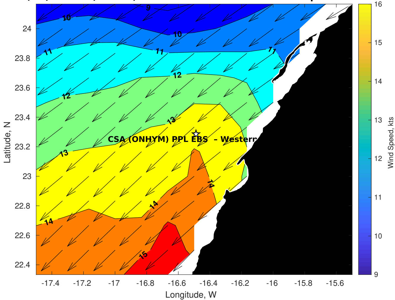
Winds (kts) for CSA (ONHYM) PPL EBS - Western Sahara at 06-Apr-2025 09:00:00
