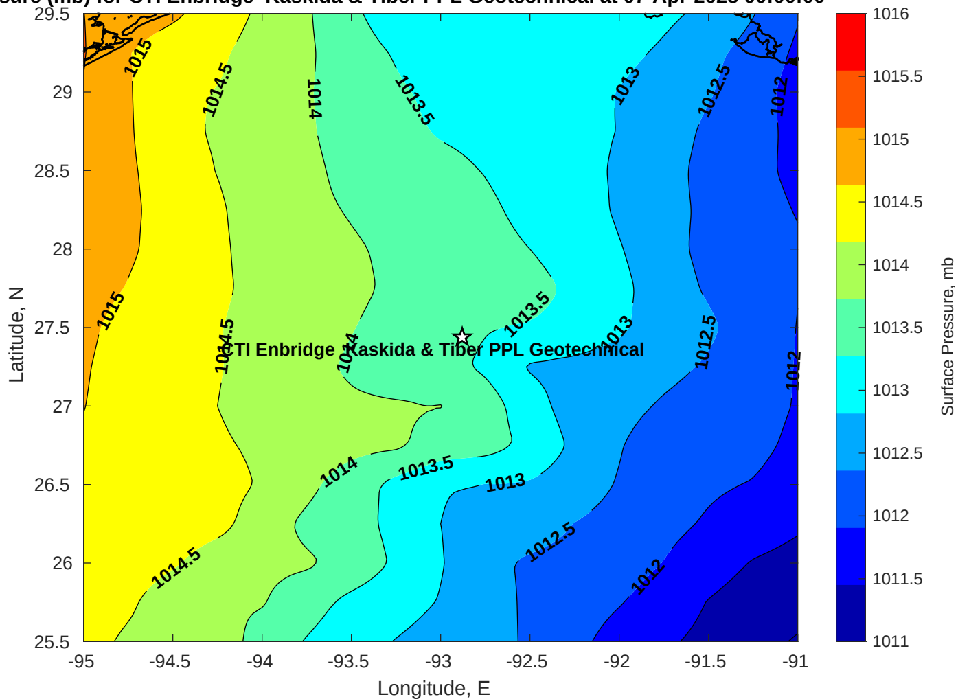
Surface Pressure (mb) for CTI Enbridge Kaskida & Tiber PPL Geotechnical at 07-Apr-2025 00:00:00
