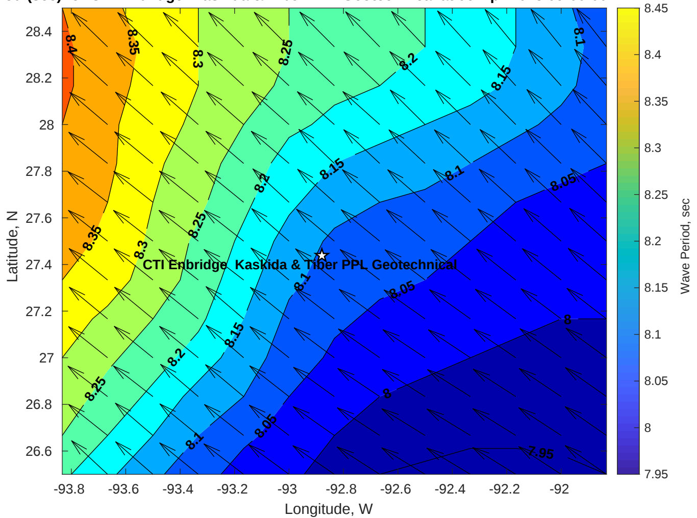
Wave Period (sec) for CTI Enbridge Kaskida & Tiber PPL Geotechnical at 06-Apr-2025 09:00:00
