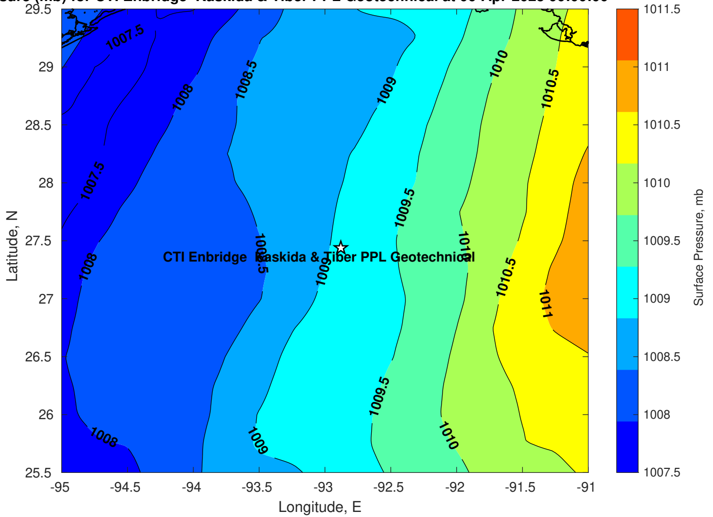
Surface Pressure (mb) for CTI Enbridge Kaskida & Tiber PPL Geotechnical at 06-Apr-2025 00:00:00
