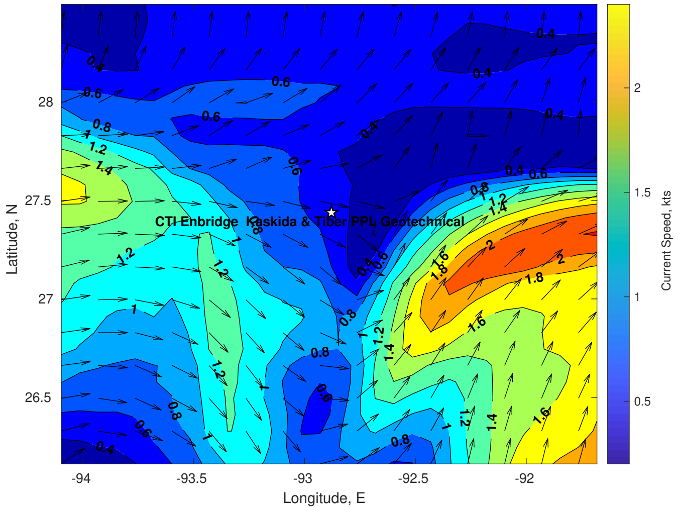
Surface Currents for CTI Enbridge Kaskida & Tiber PPL Geotechnical at 05-Apr-2025 00:00:00
