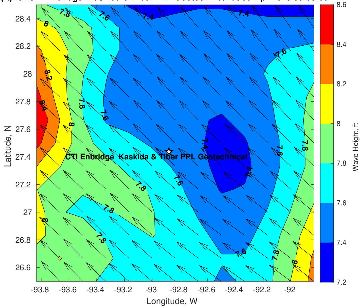
Wave Height (ft) for CTI Enbridge Kaskida & Tiber PPL Geotechnical at 06-Apr-2025 09:00:00
