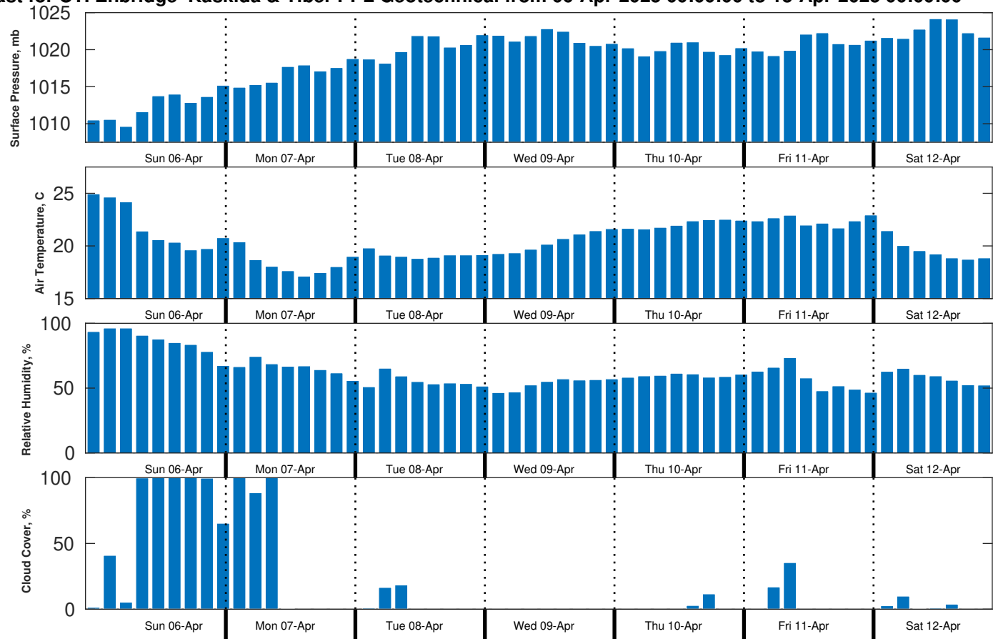
Met Forecast for CTI Enbridge Kaskida & Tiber PPL Geotechnical from 06-Apr-2025 00:00:00 to 13-Apr-2025 00:00:00
