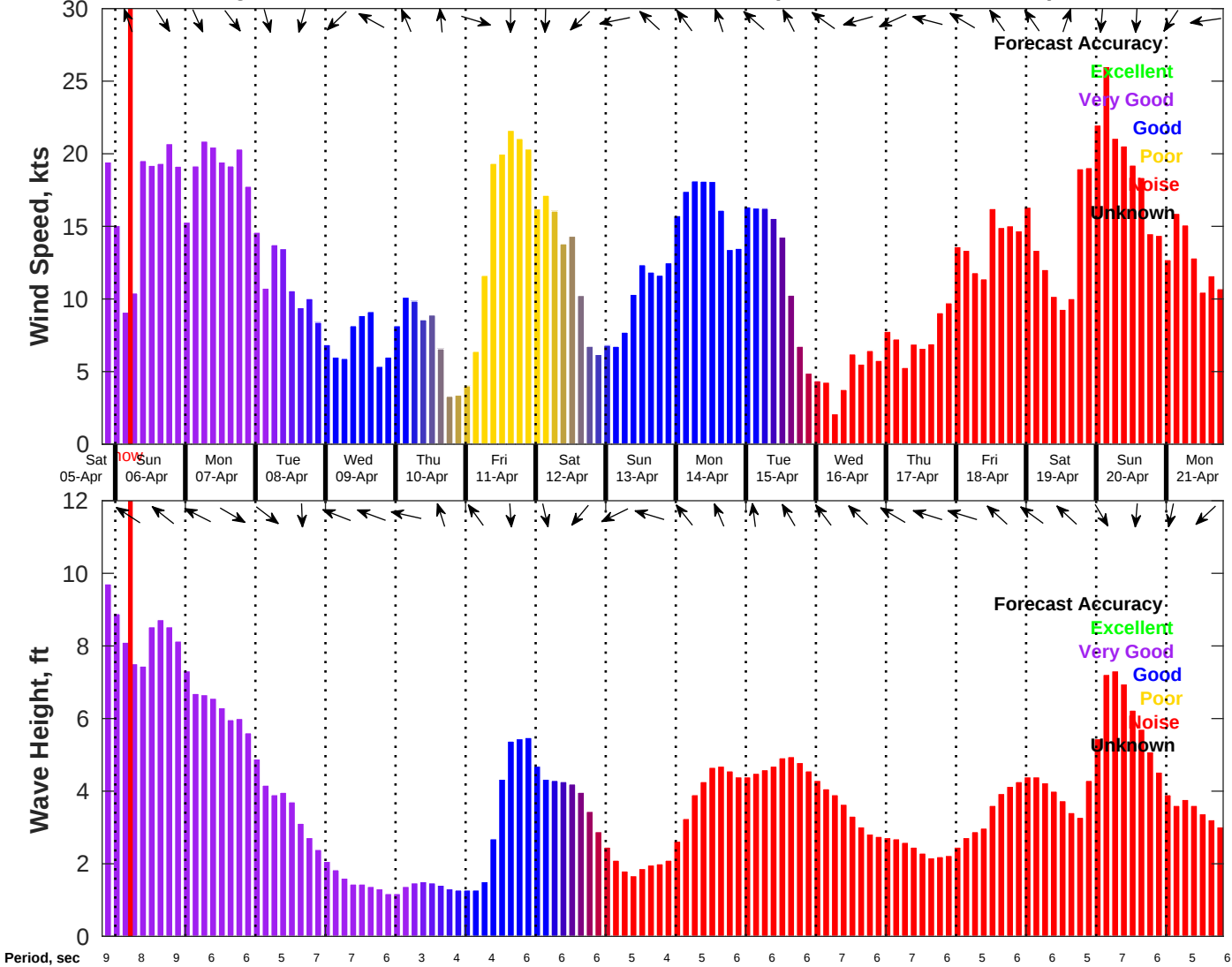
Wind & Wave Forecast for CTI Enbridge Kaskida & Tiber PPL Geotechnical from 05-Apr-2025 20:00:00 to 21-Apr-2025 20:00:00
