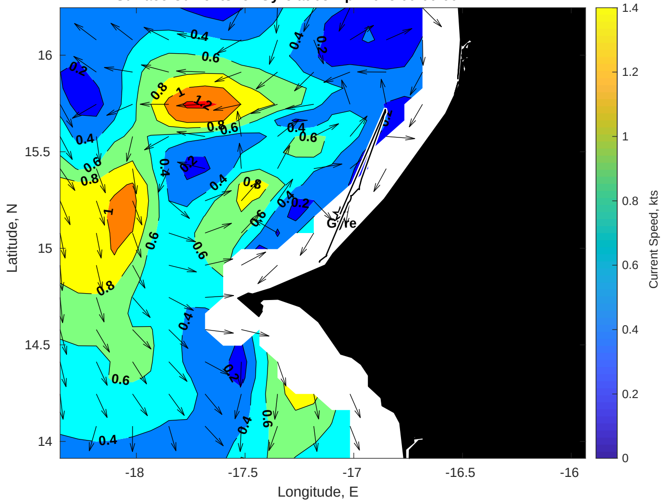
Surface Currents for Gyre at 05-Apr-2025 00:00:00
