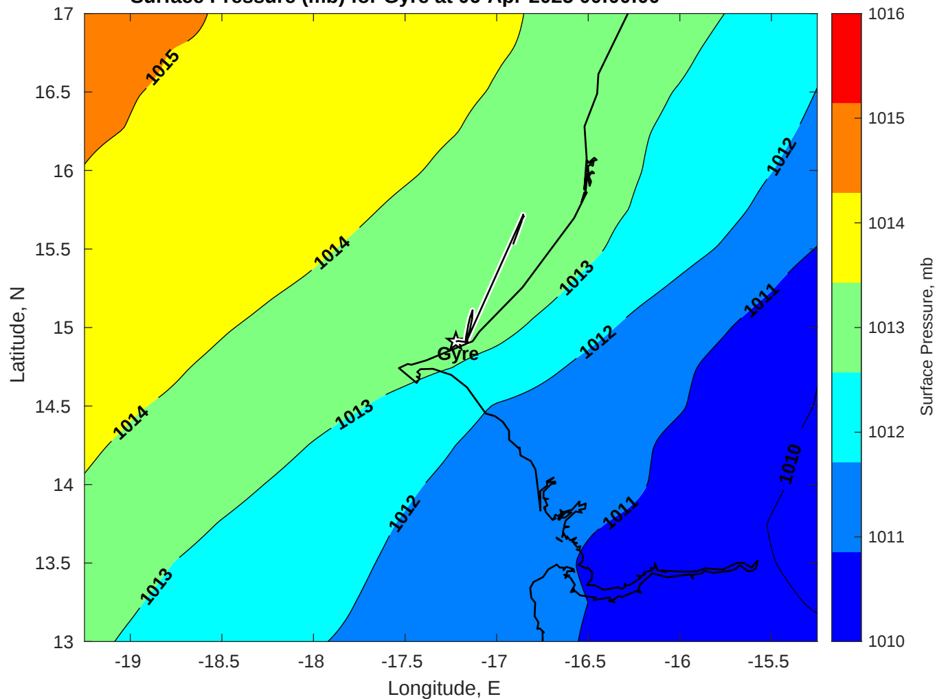
Surface Pressure (mb) for Gyre at 06-Apr-2025 00:00:00
