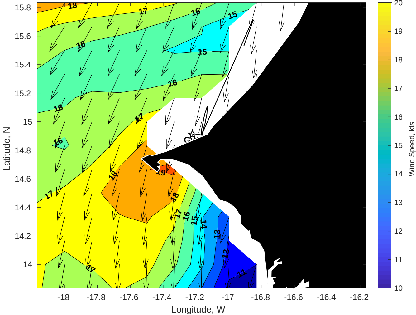
Winds (kts) for Gyre at 06-Apr-2025 09:00:00
