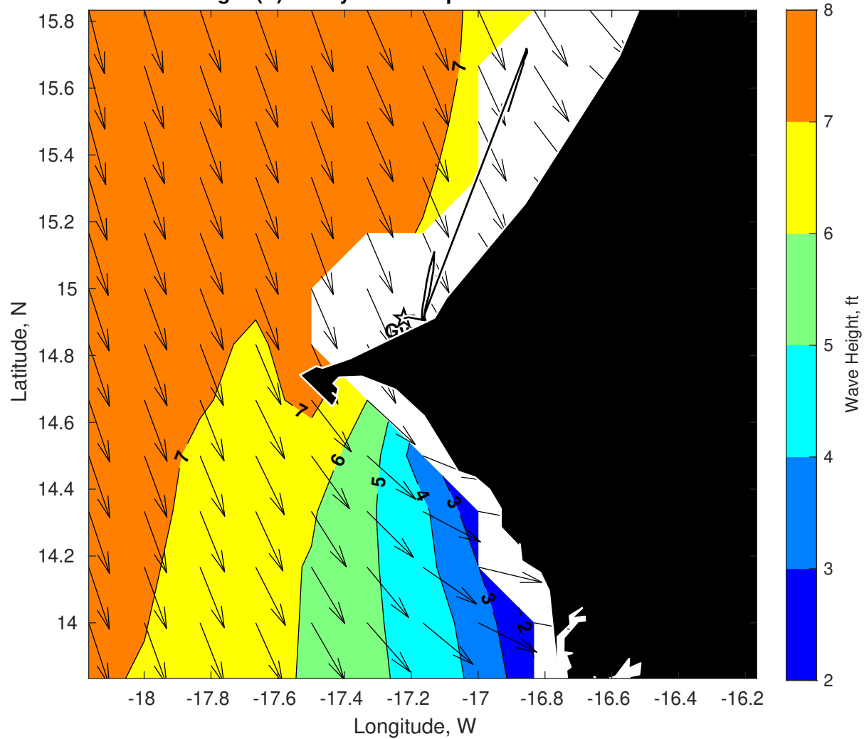
Wave Height (ft) for Gyre at 06-Apr-2025 09:00:00
