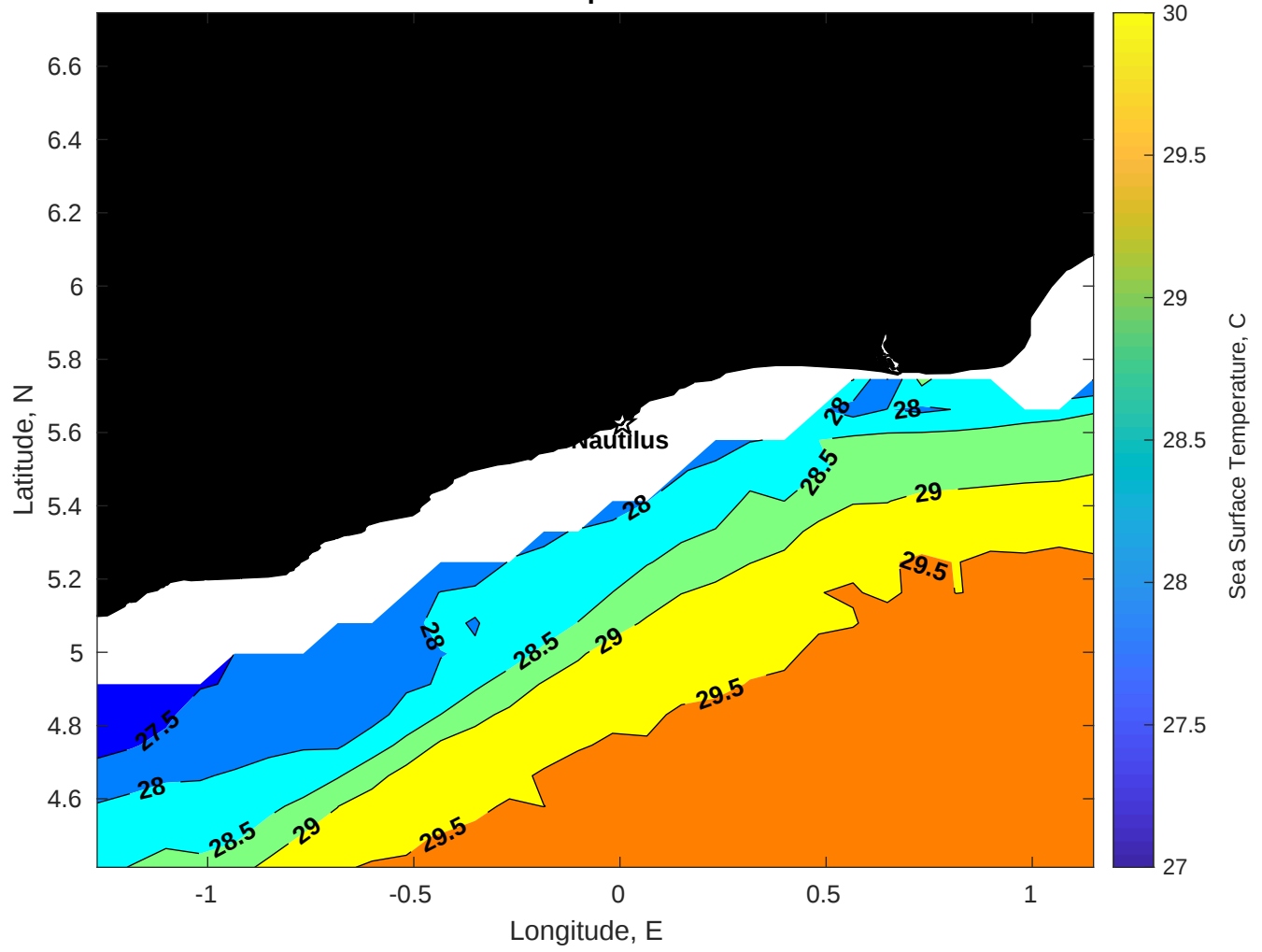
SST for Nautilus at 05-Apr-2025 00:00:00
