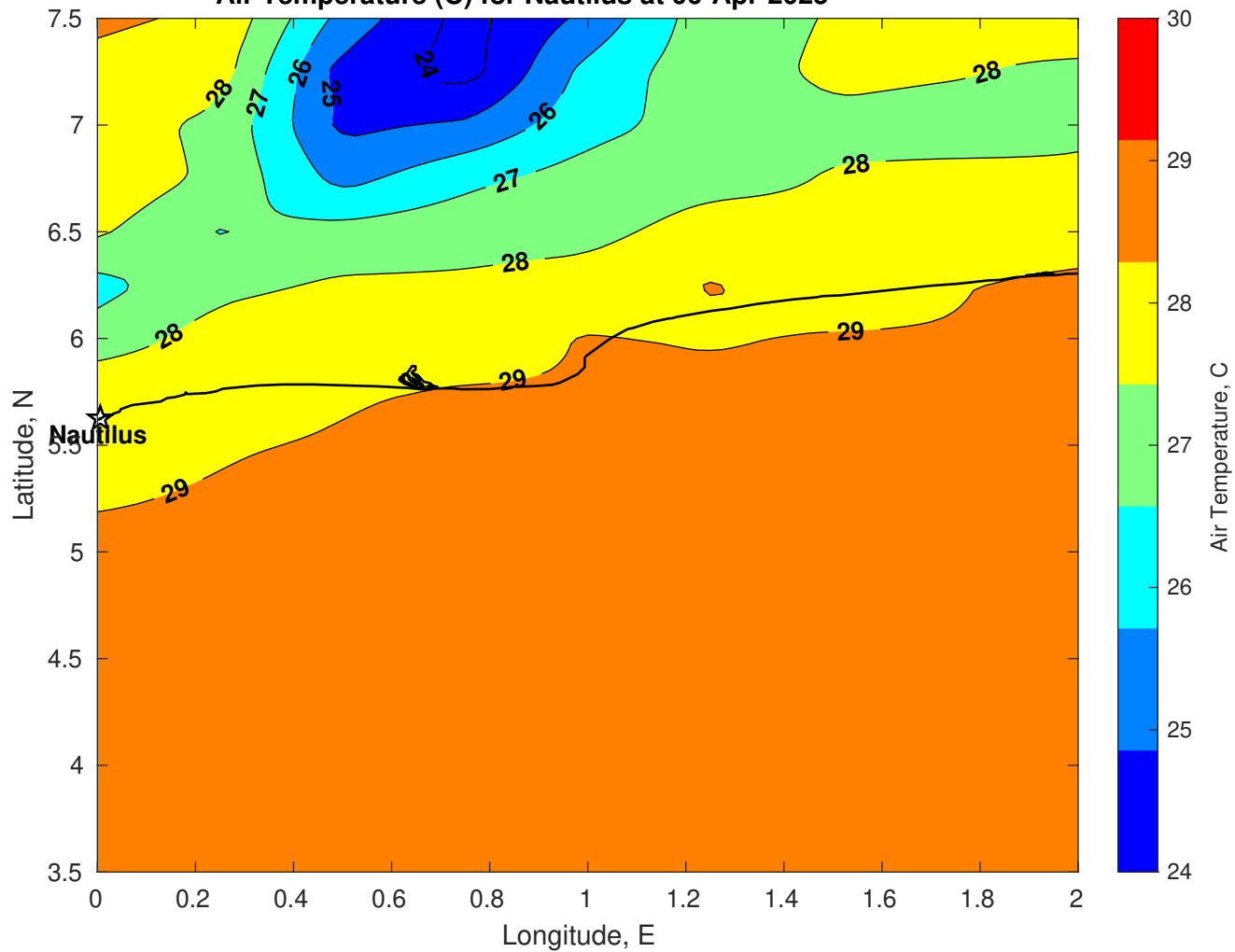
Air Temperature (C) for Nautilus at 06-Apr-2025
