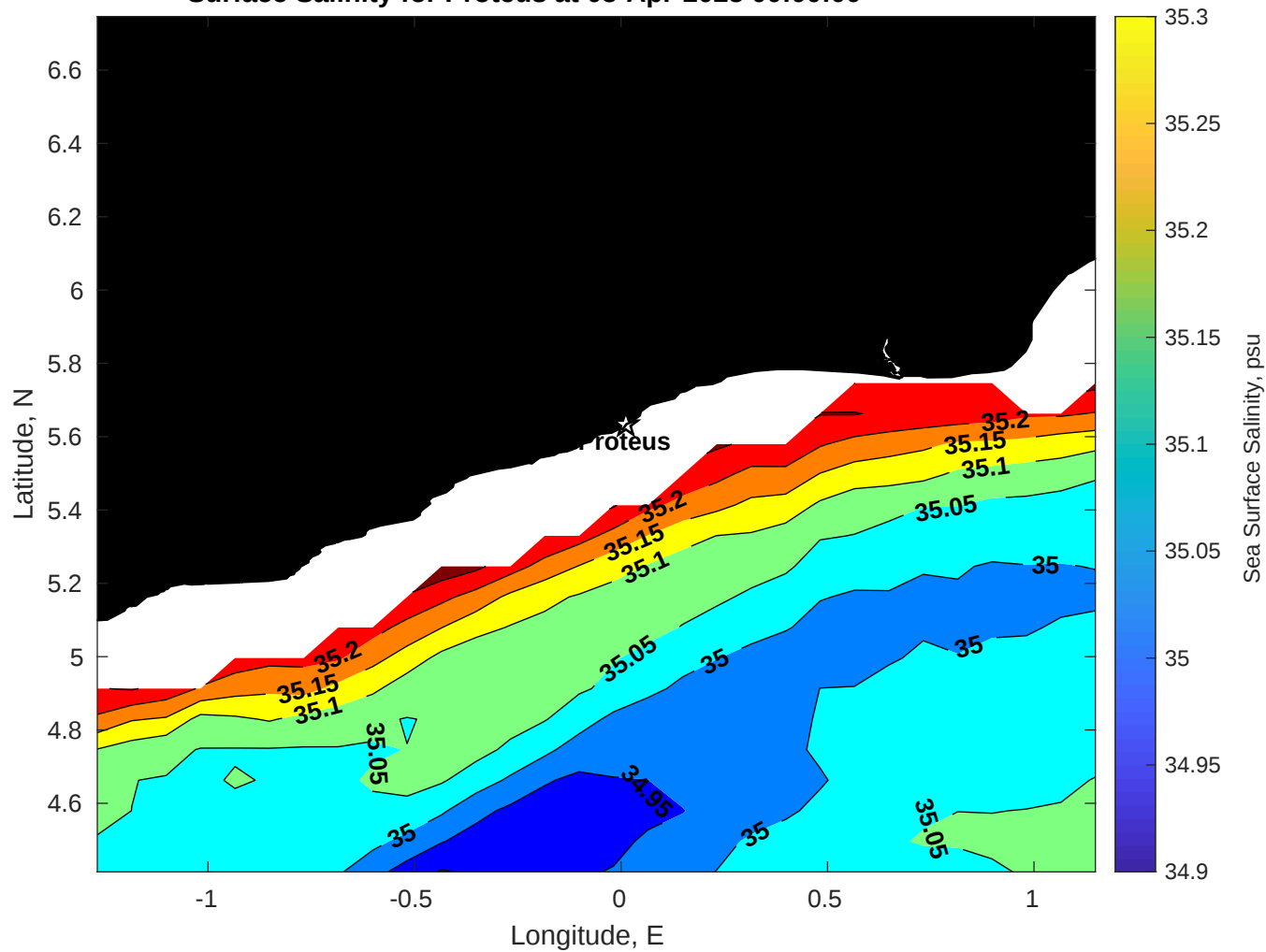
Surface Salinity for Proteus at 05-Apr-2025 00:00:00
