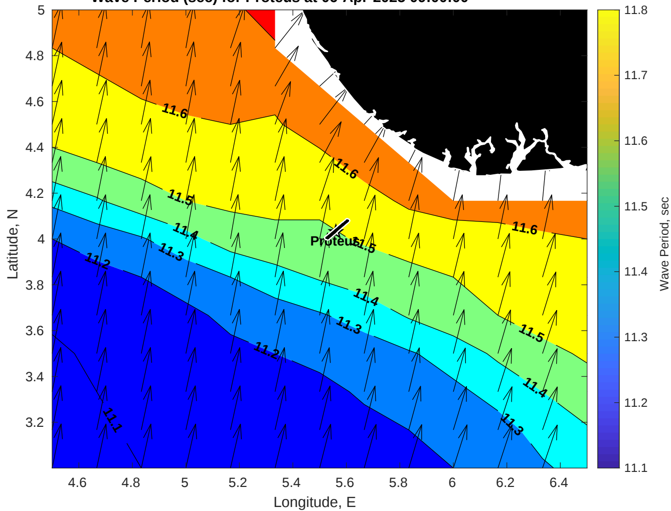
Wave Period (sec) for Proteus at 06-Apr-2025 09:00:00
