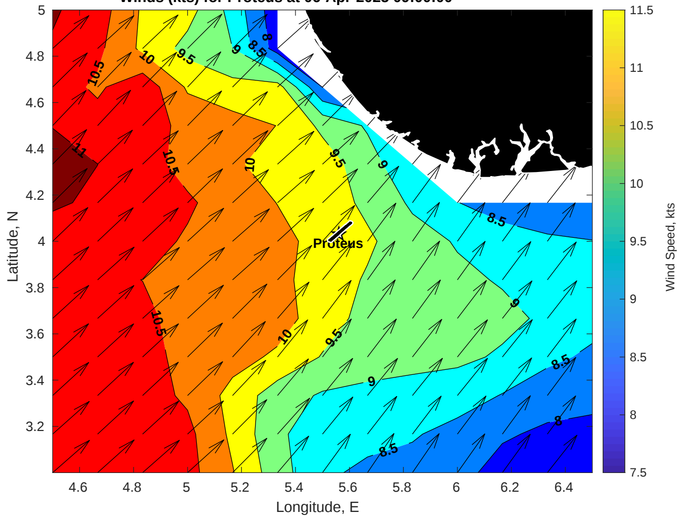
Winds (kts) for Proteus at 06-Apr-2025 09:00:00
