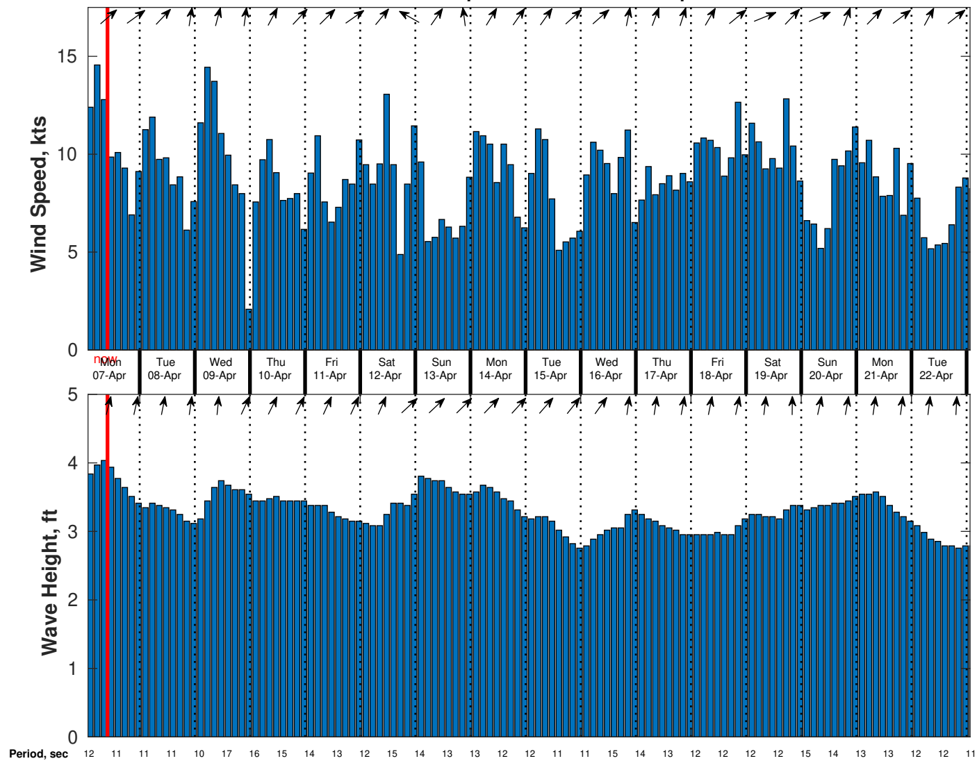
Wind & Wave Forecast for Proteus from 06-Apr-2025 01:00:00 to 22-Apr-2025 01:00:00
