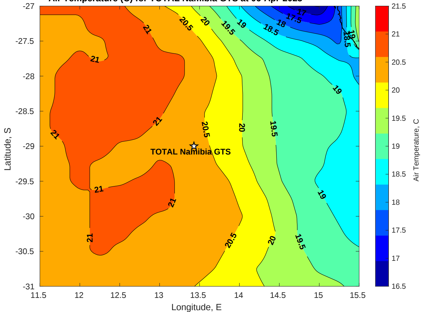
Air Temperature (C) for TOTAL Namibia GTS at 06-Apr-2025
