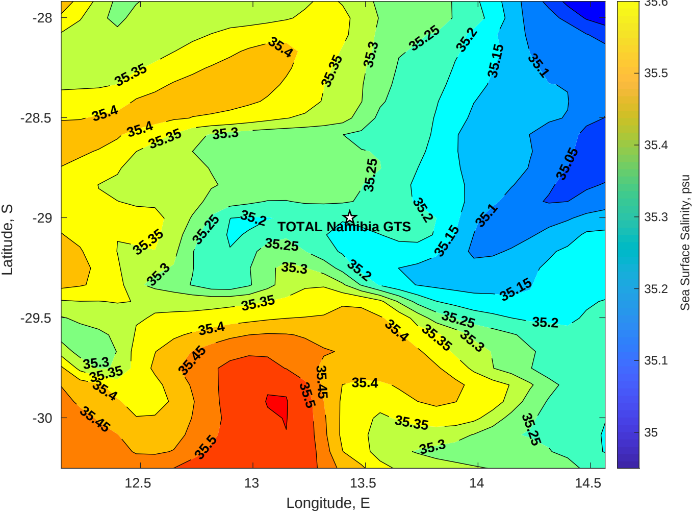
Surface Salinity for TOTAL Namibia GTS at 05-Apr-2025 00:00:00
