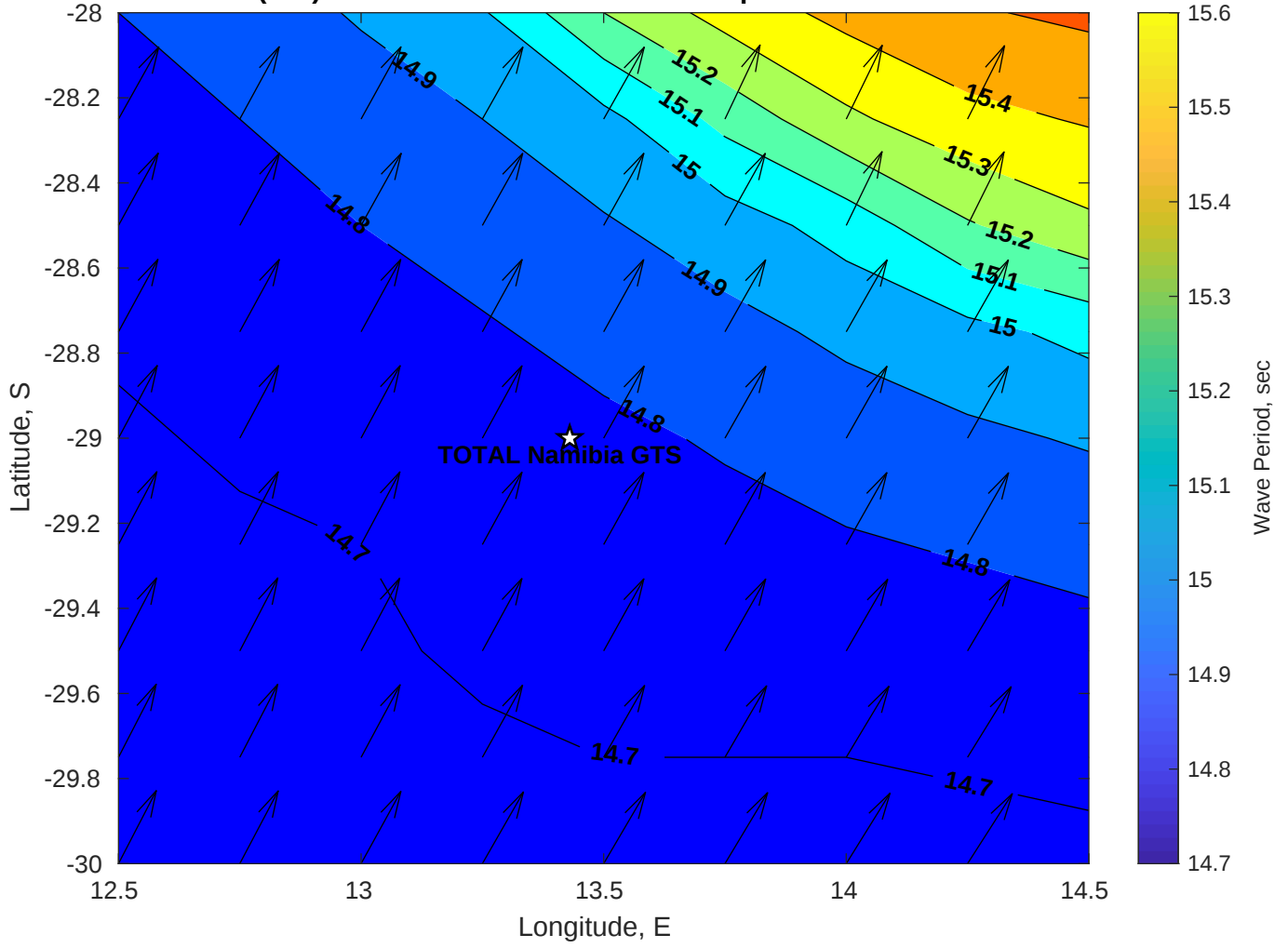
Wave Period (sec) for TOTAL Namibia GTS at 06-Apr-2025 09:00:00
