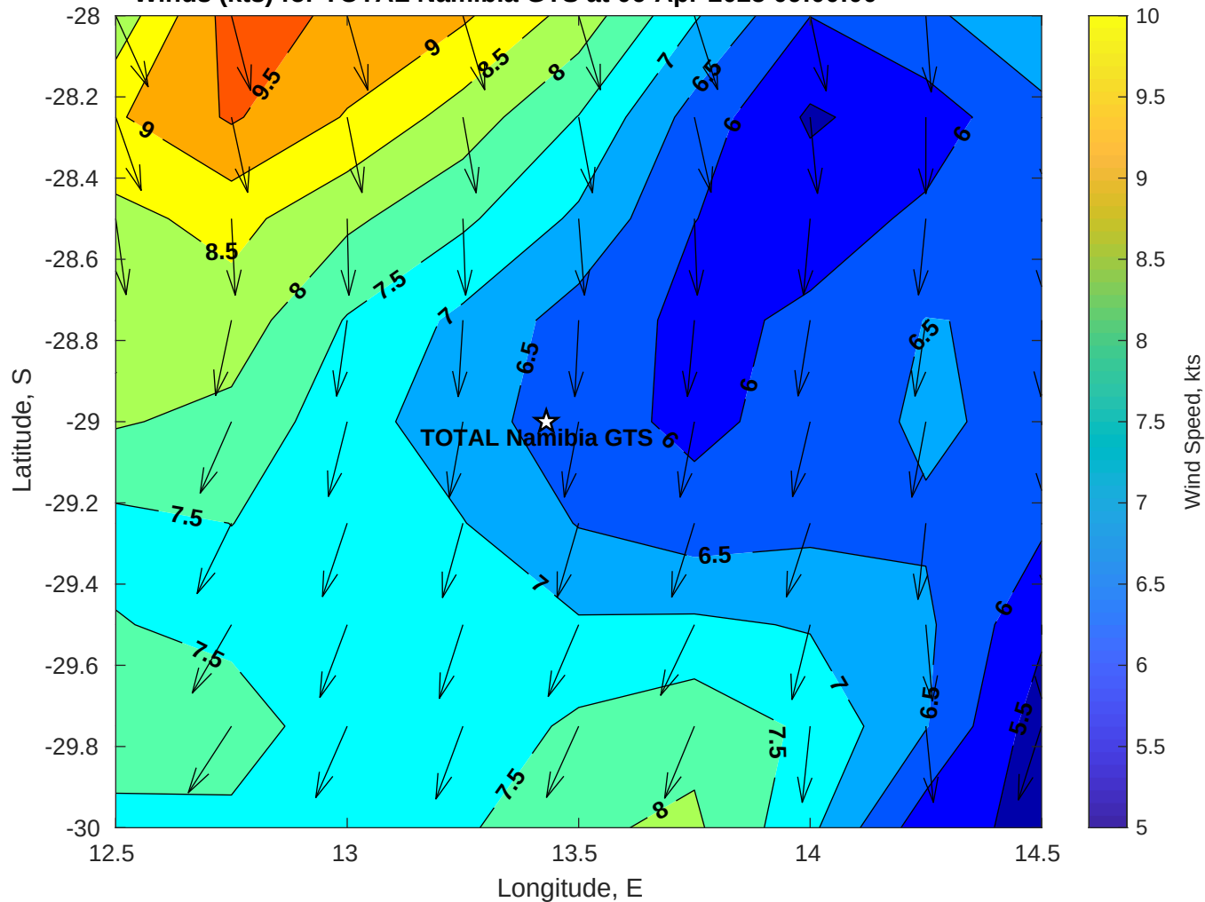
Winds (kts) for TOTAL Namibia GTS at 06-Apr-2025 09:00:00
