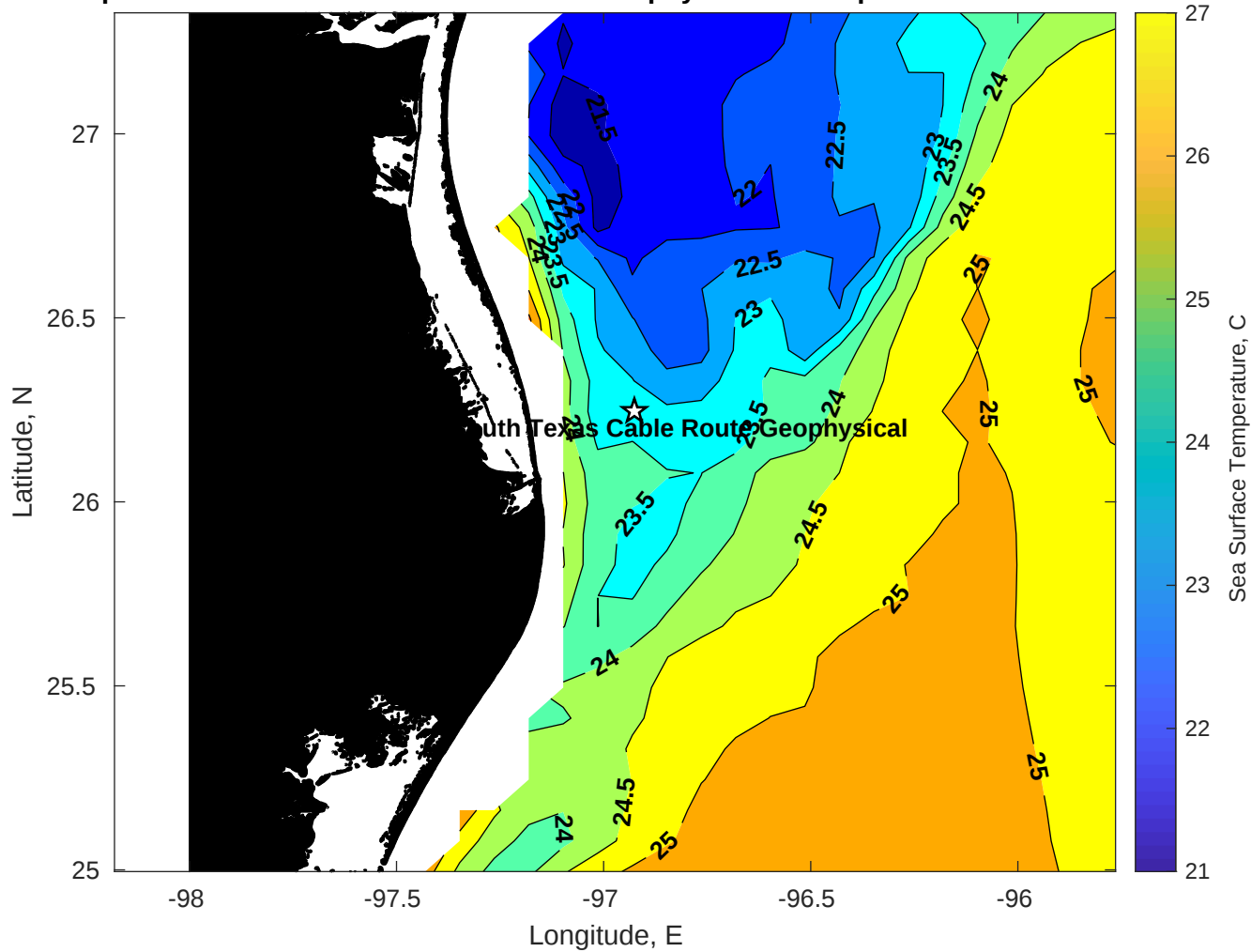
SST for Tampnet P2378 South Texas Cable Route Geophysical at 05-Apr-2025 00:00:00
