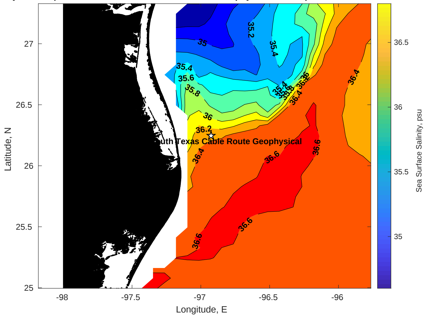
Surface Salinity for Tampnet P2378 South Texas Cable Route Geophysical at 05-Apr-2025 00:00:00
