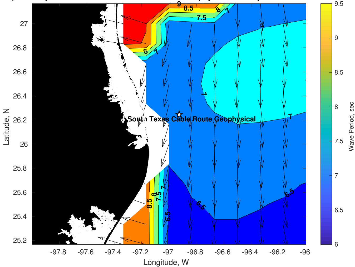
Period (sec) for Tampnet P2378 South Texas Cable Route Geophysical at 06-Apr-2025 09:00:00
