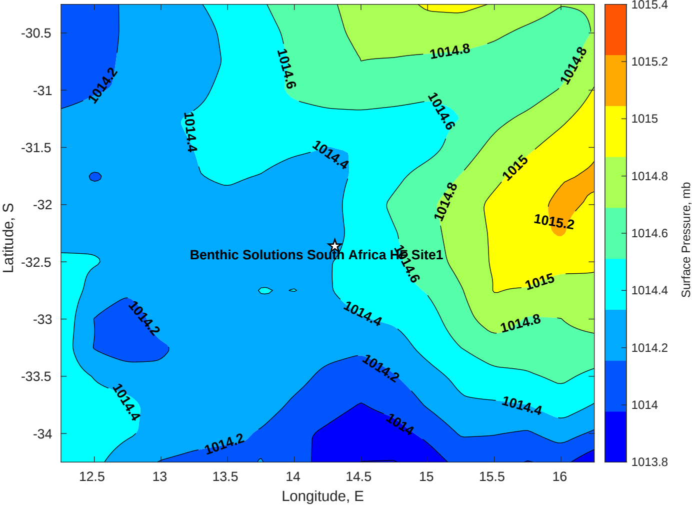
Surface Pressure (mb) for Benthic Solutions South Africa HF Site1 at 08-Apr-2025 00:00:00
