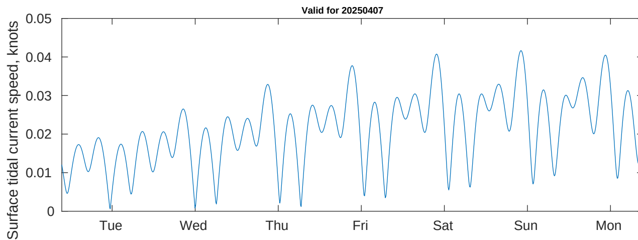
Tidal Currents and Heights for Benthic Solutions South Africa HF Site1 at 20250407
