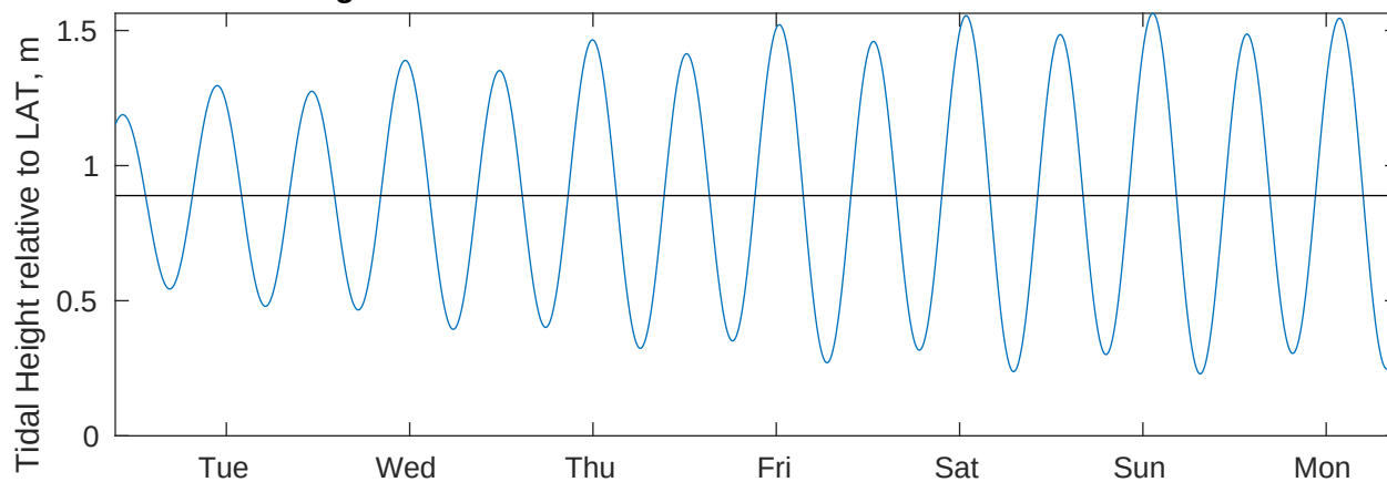
Tidal Currents and Heights for Benthic Solutions South Africa HF Site1 at 20250407
