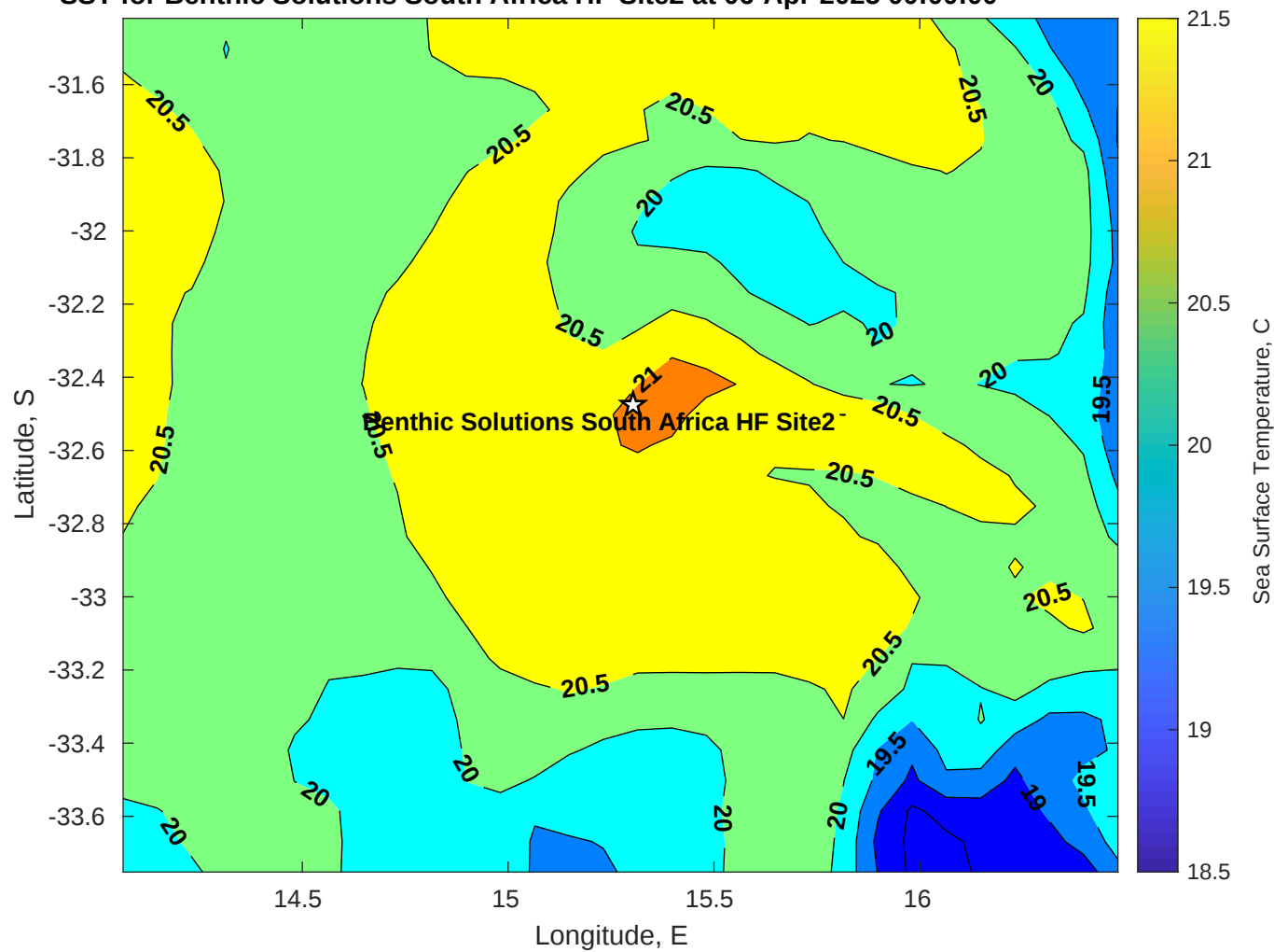
SST for Benthic Solutions South Africa HF Site2 at 06-Apr-2025 00:00:00
