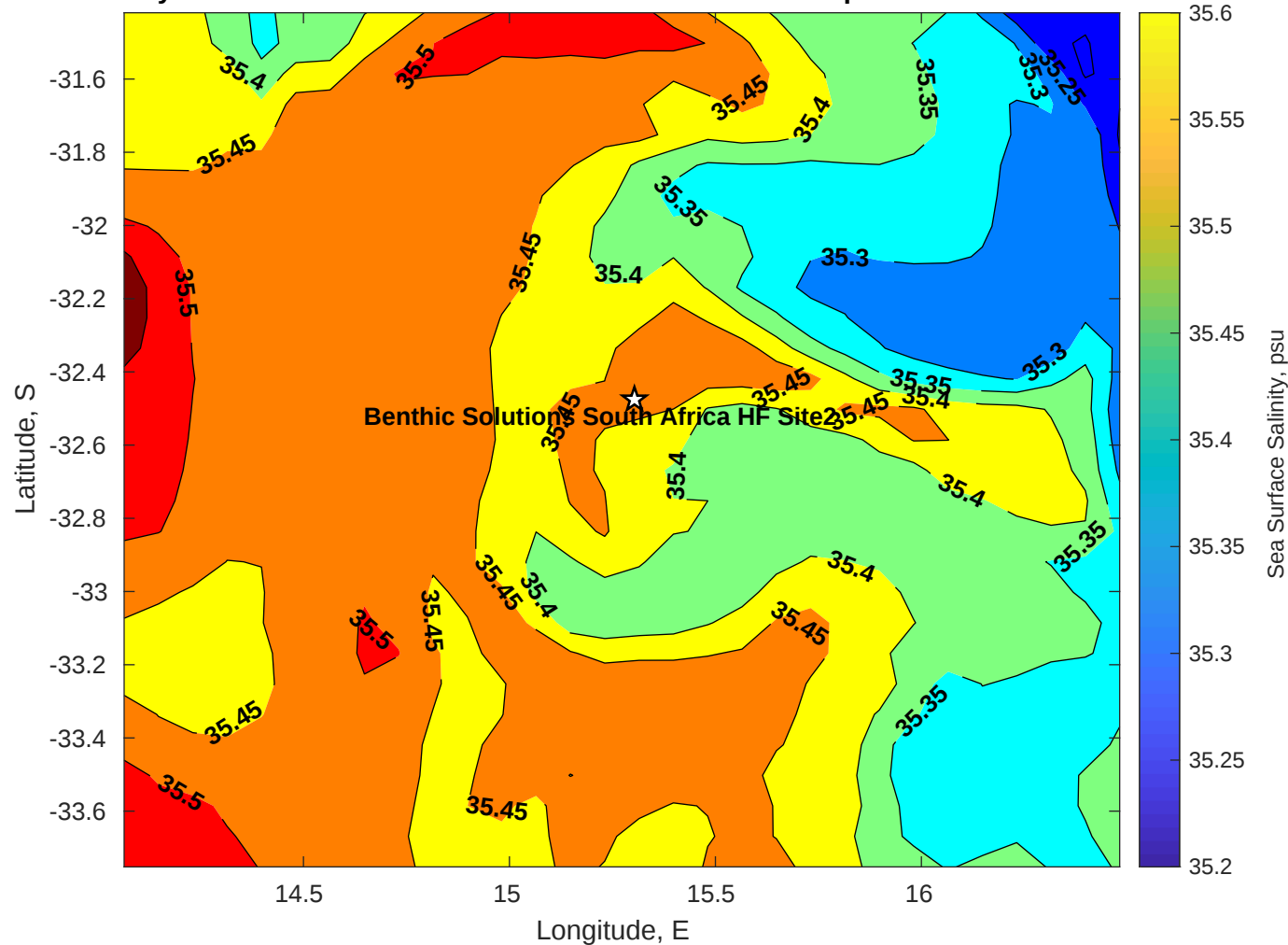
Surface Salinity for Benthic Solutions South Africa HF Site2 at 06-Apr-2025 00:00:00
